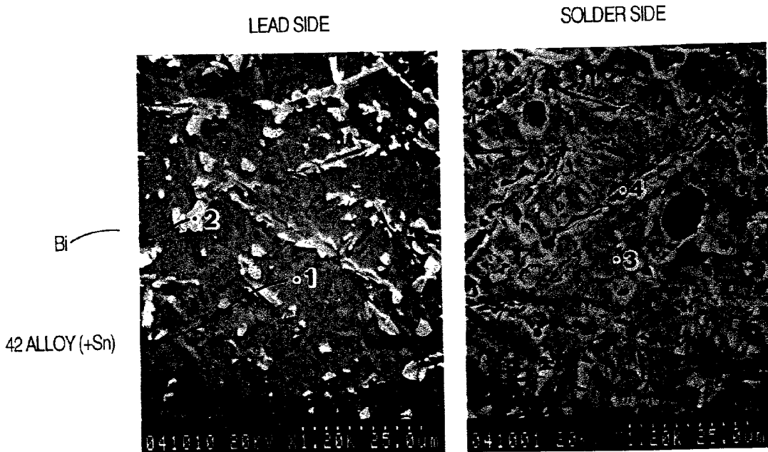
(b) FRACTURED PORTION
