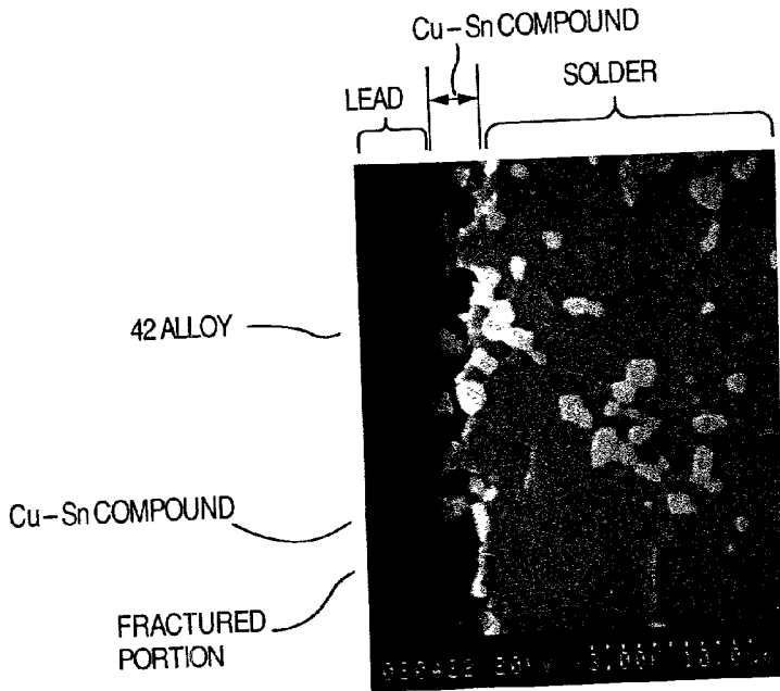
(a) SECTIONAL VIEW
