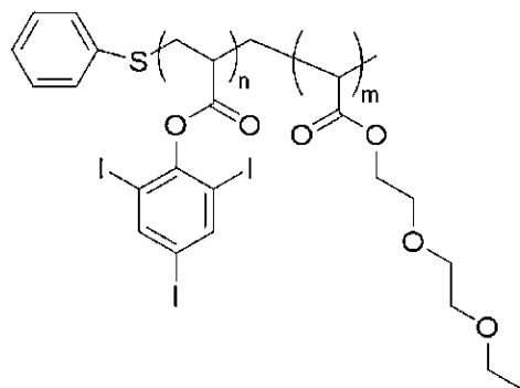
BT-poly(TIP-AC-co-EEA)
