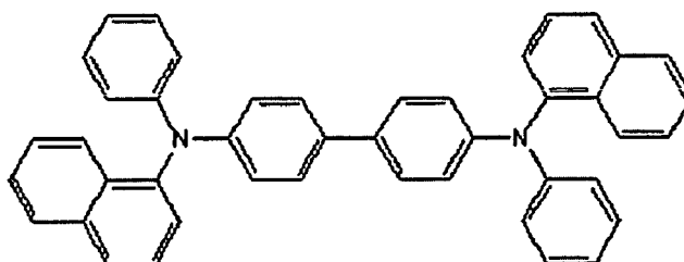
NPB
