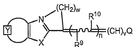
Formula VII
