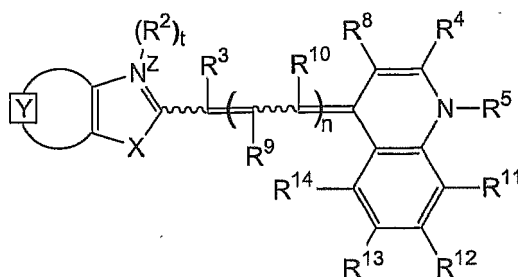
Formula II
