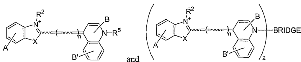
Formula VIa
