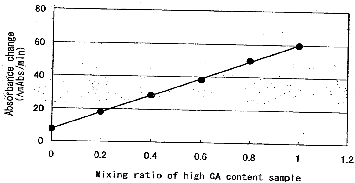
Fig. 3 Linearity in GA assay
