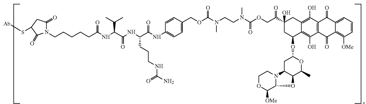
PNU-159682-val-cit-PAB-spacer-Ab
