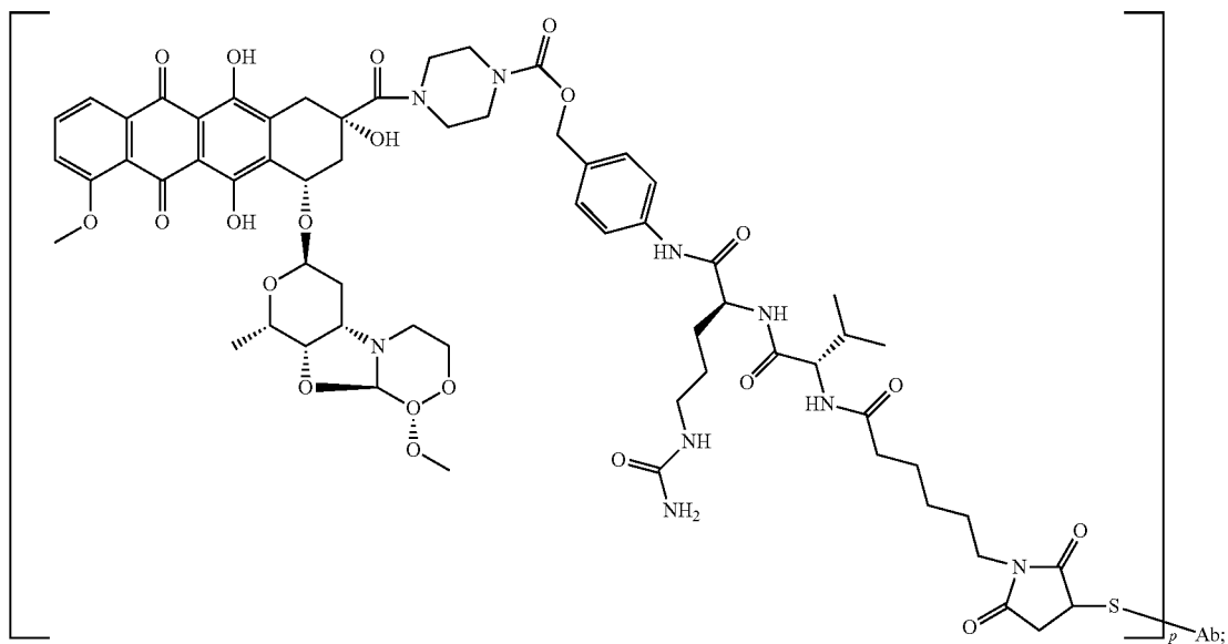
PNU-159682-val-cit-PAB-Ab
