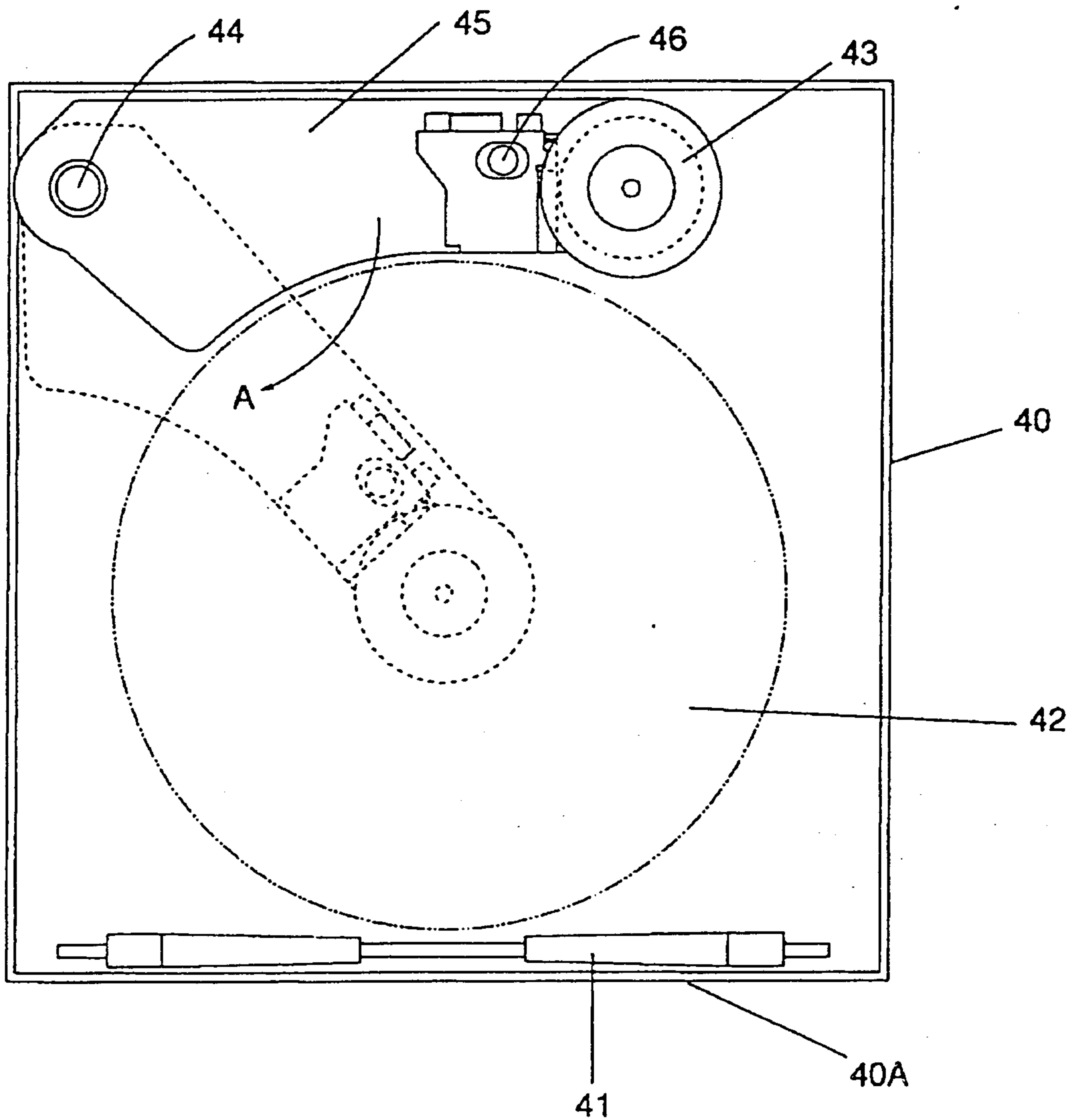
FIG. 1 PRIOR ART
