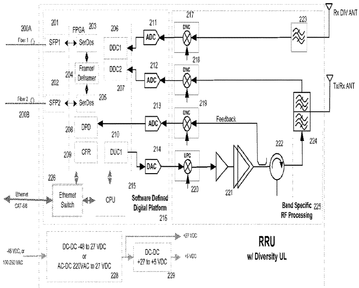
FIG. 2: Remote Radio Head Unit
