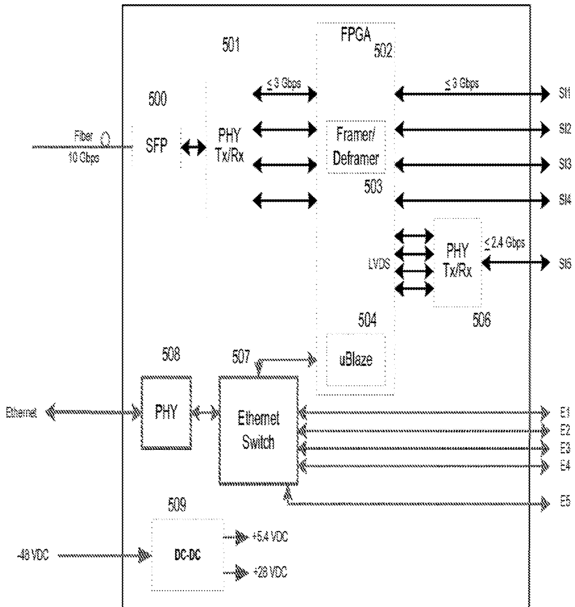
FIG. 5: Remote Radio Head Unit Access Module
