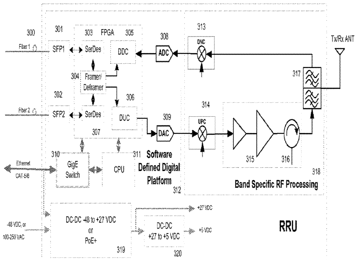
FIG. 3: Remote Radio Head Unit
