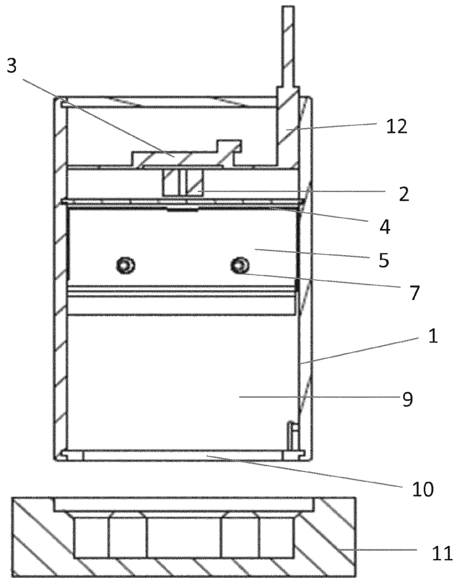
Section B-B
