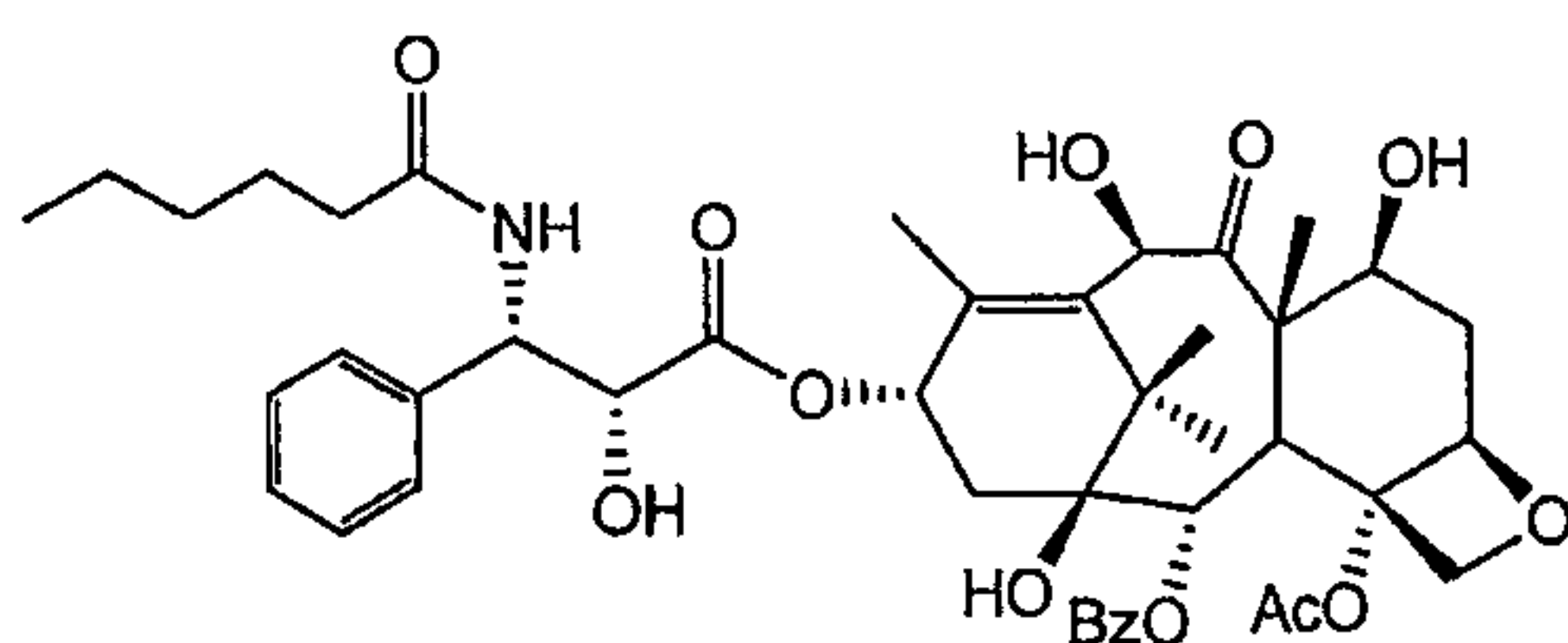
10-Deacetyltaxol C
