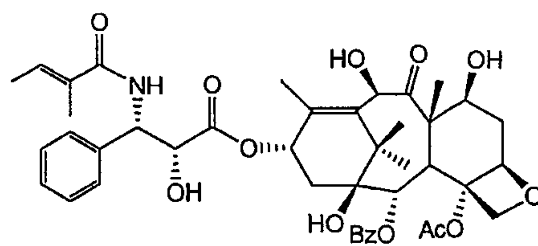
10-Deacetyltaxol B
