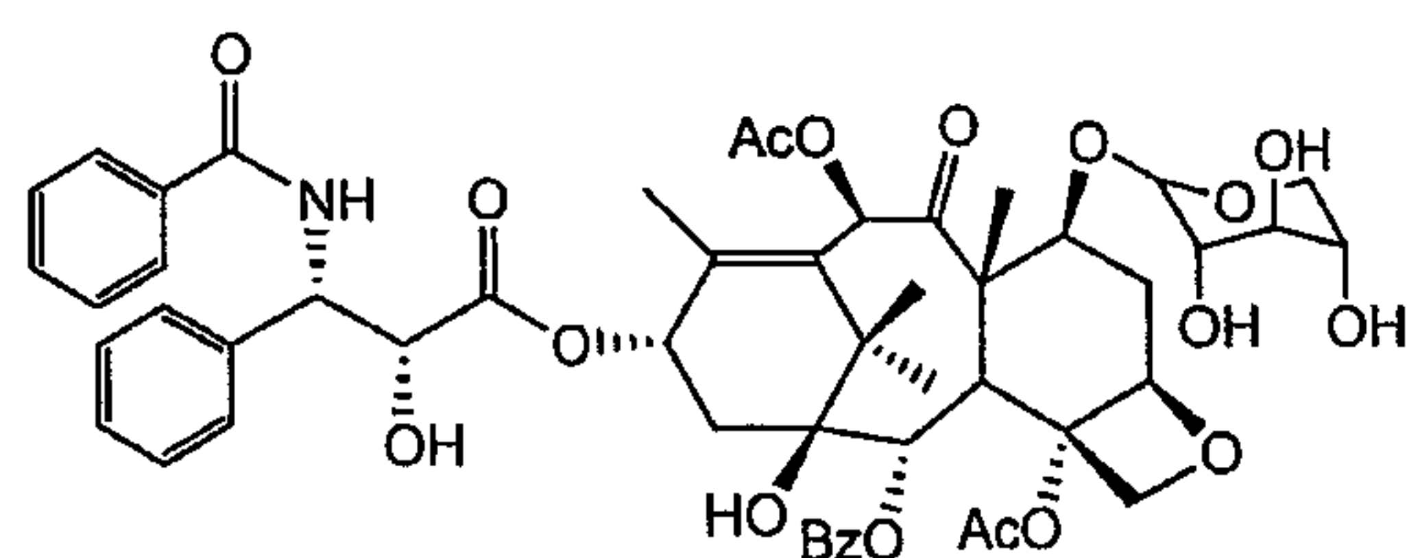
7-Xylosyltaxol A
