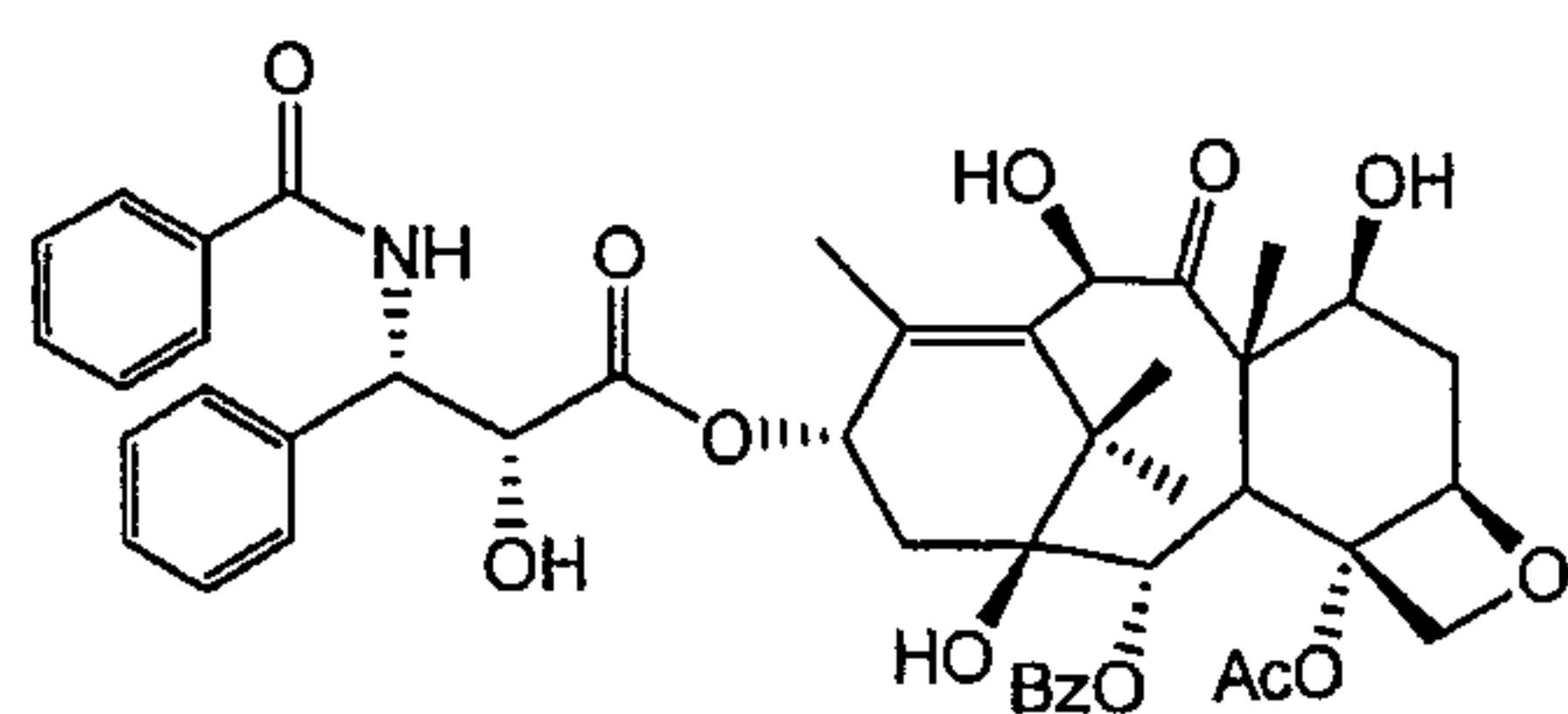
10-Deacetyltaxol A
