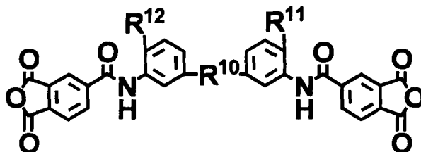
[Chemical formula 4]
