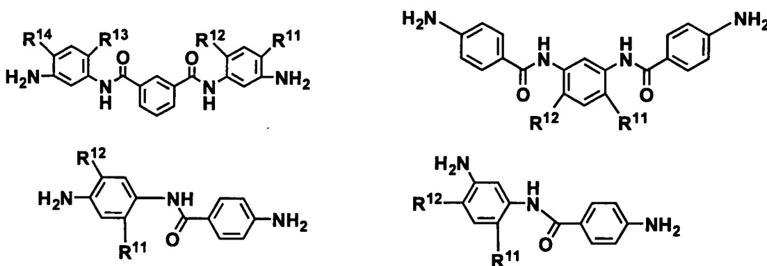
[Chemical formula 5]
