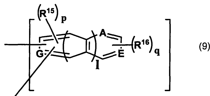
[Chemical formula 8]
