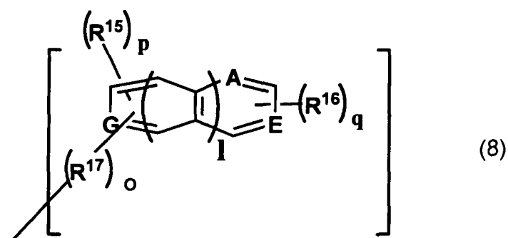
[Chemical formula 7]
