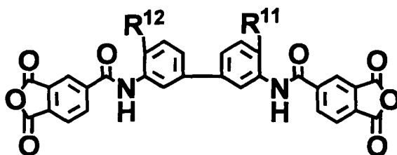
[Chemical formula 3]
