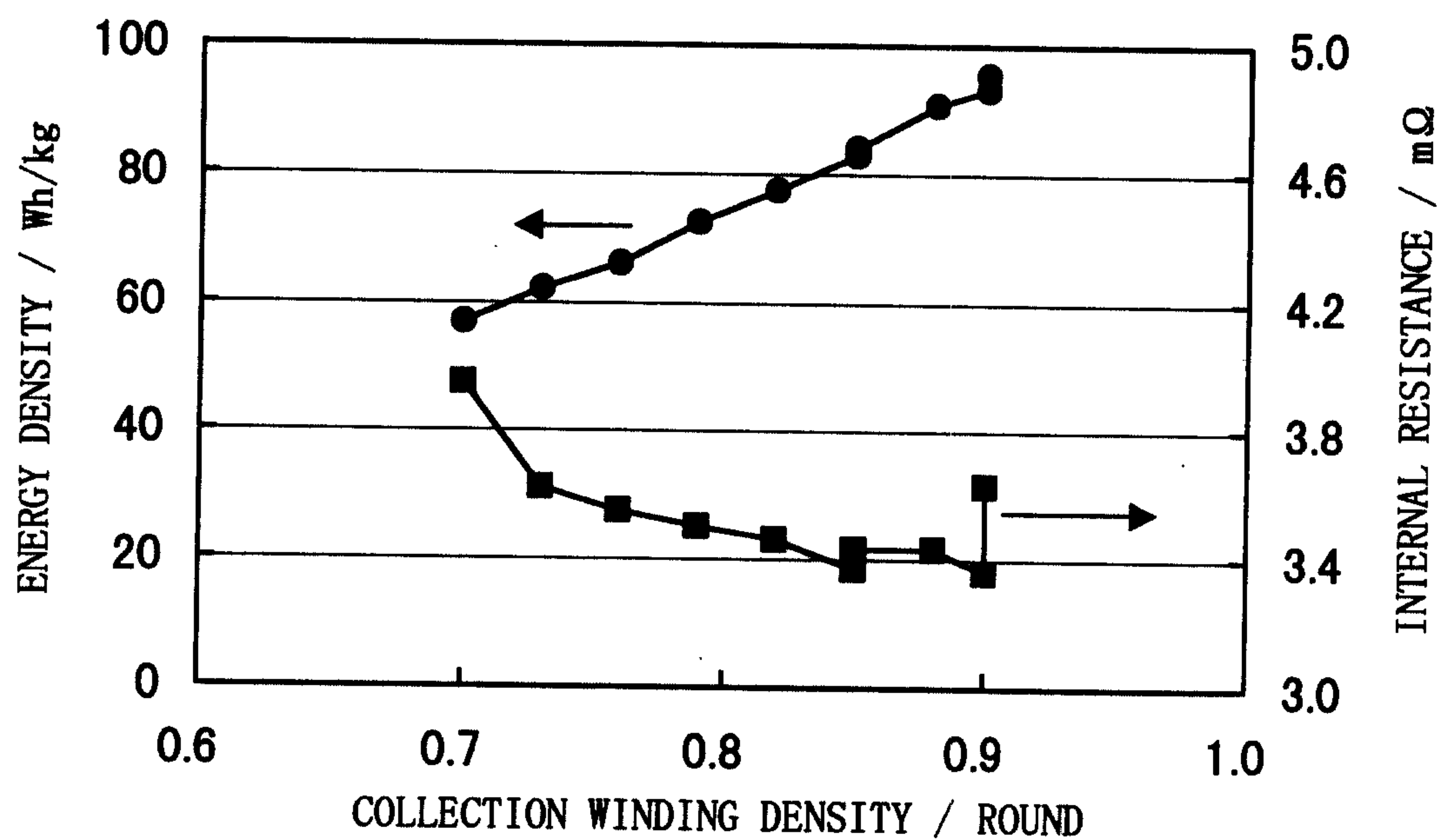
FIG. 4 (b) ONE SIDE THICKNESS OF POSITIVE ACTIVE MATERIAL LAYER : WITH 150 \mu m
