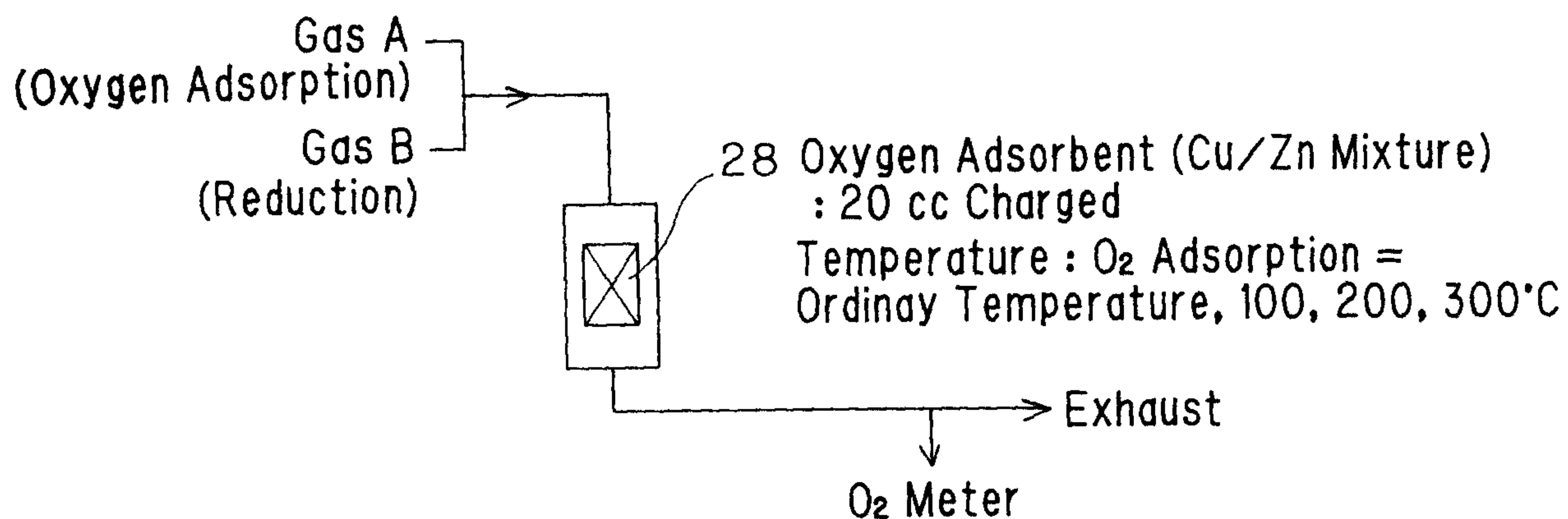
Example of Testing Device
