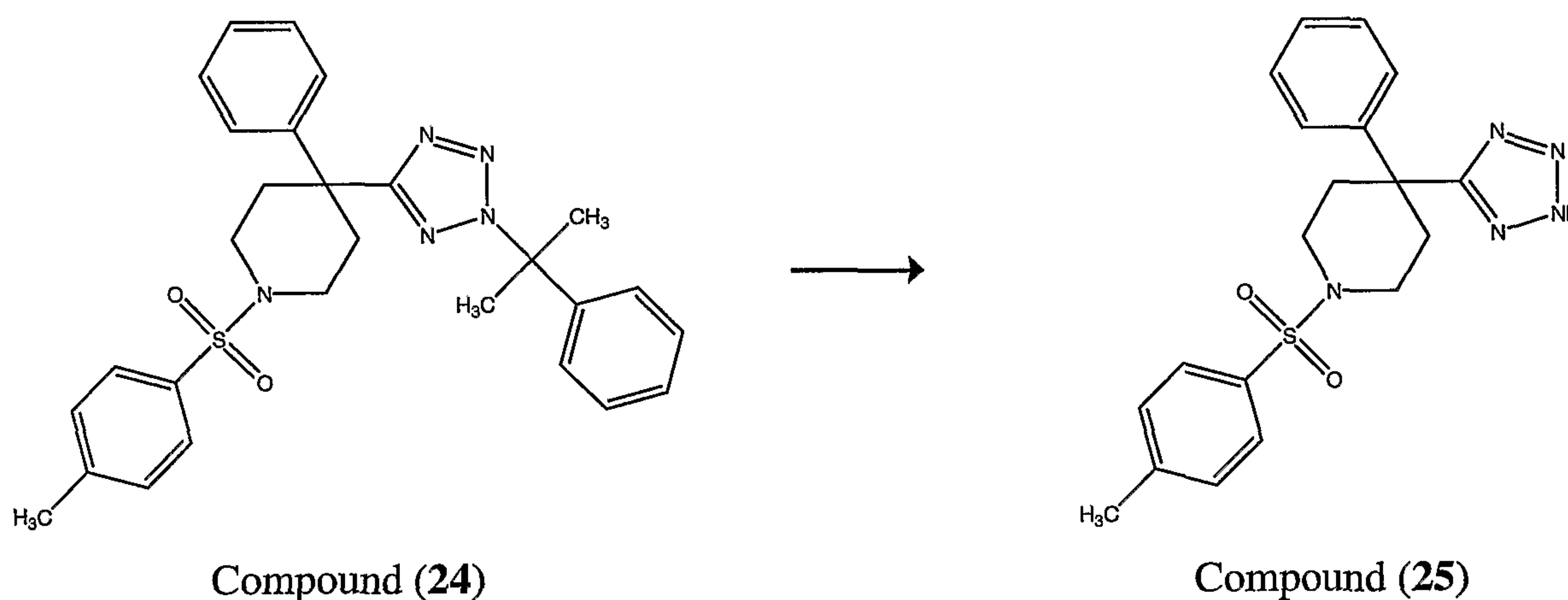
Scheme 24
