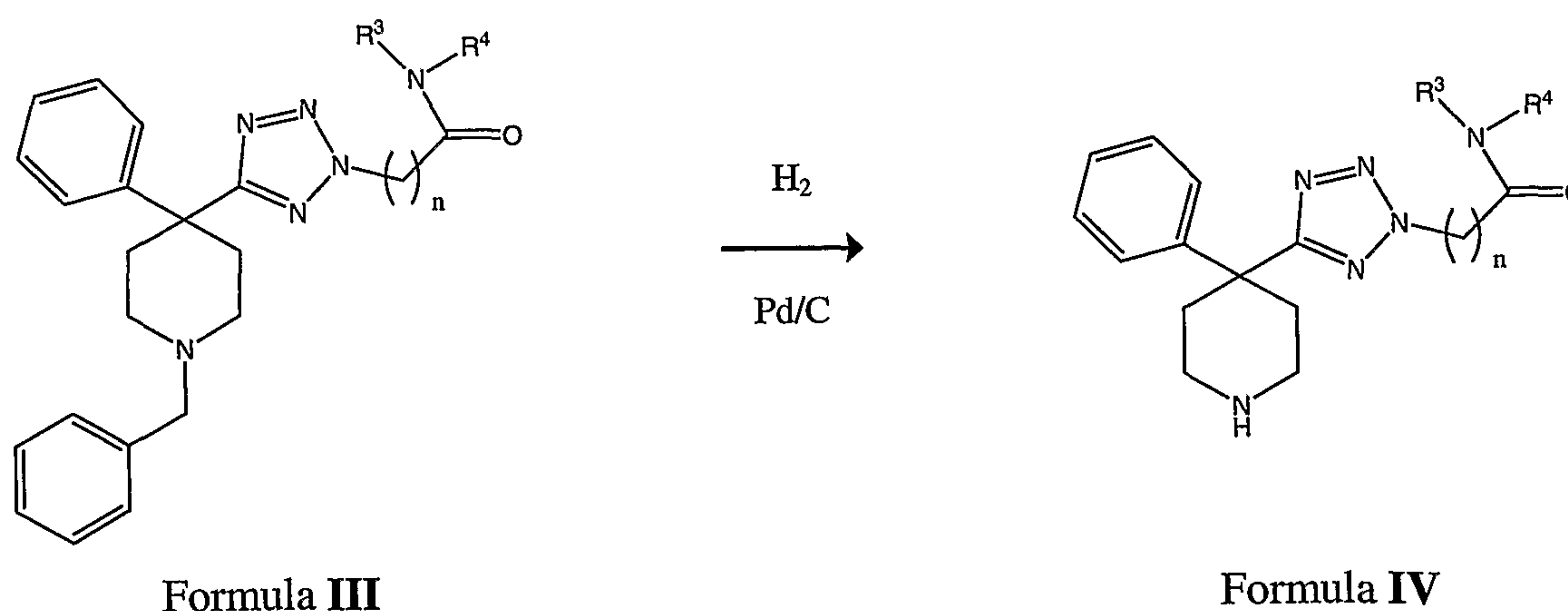
Scheme 3
