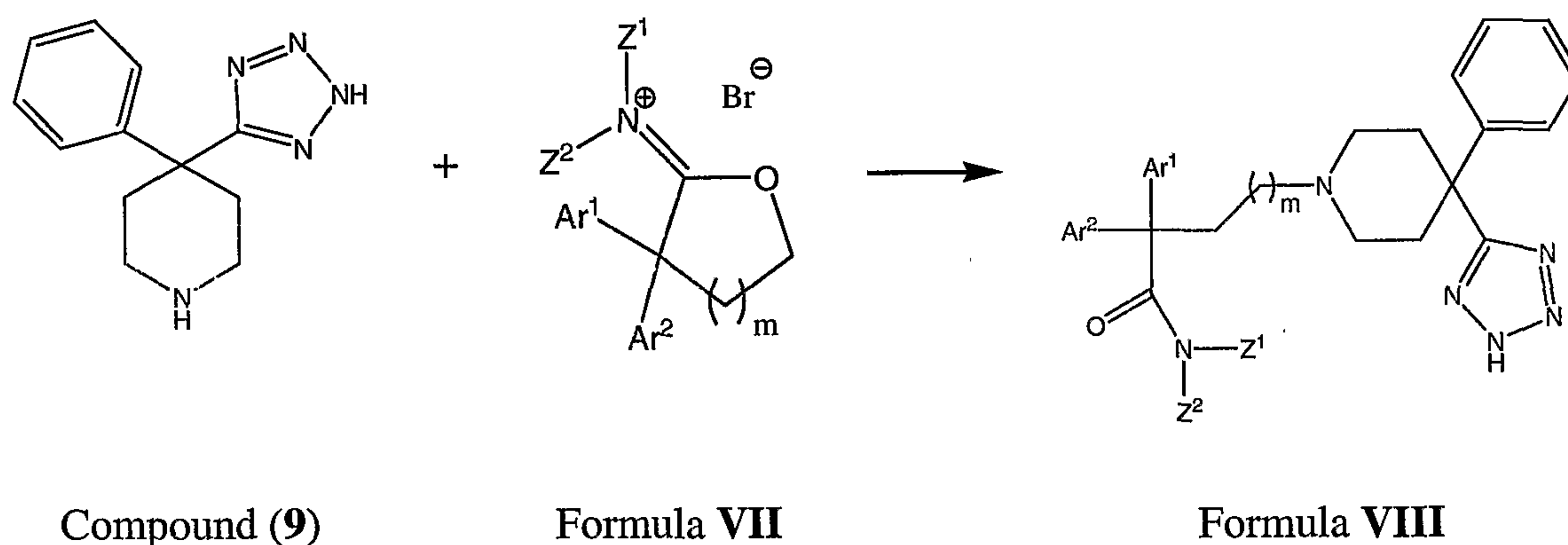
Scheme 8
