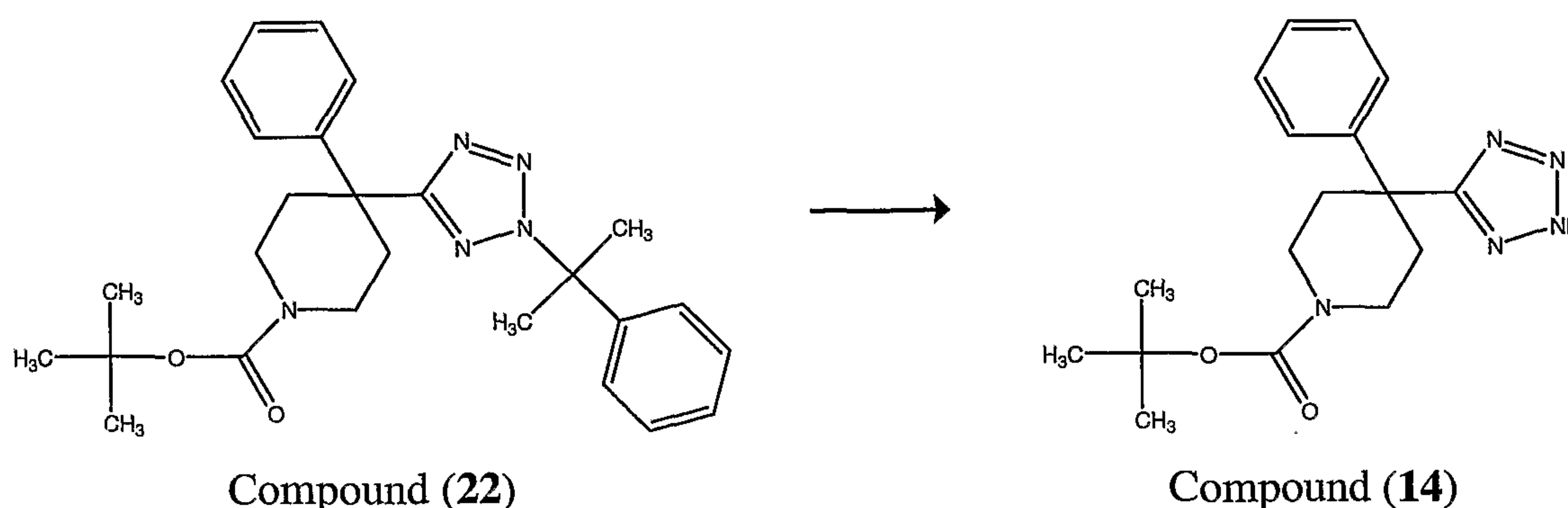
Scheme 23
