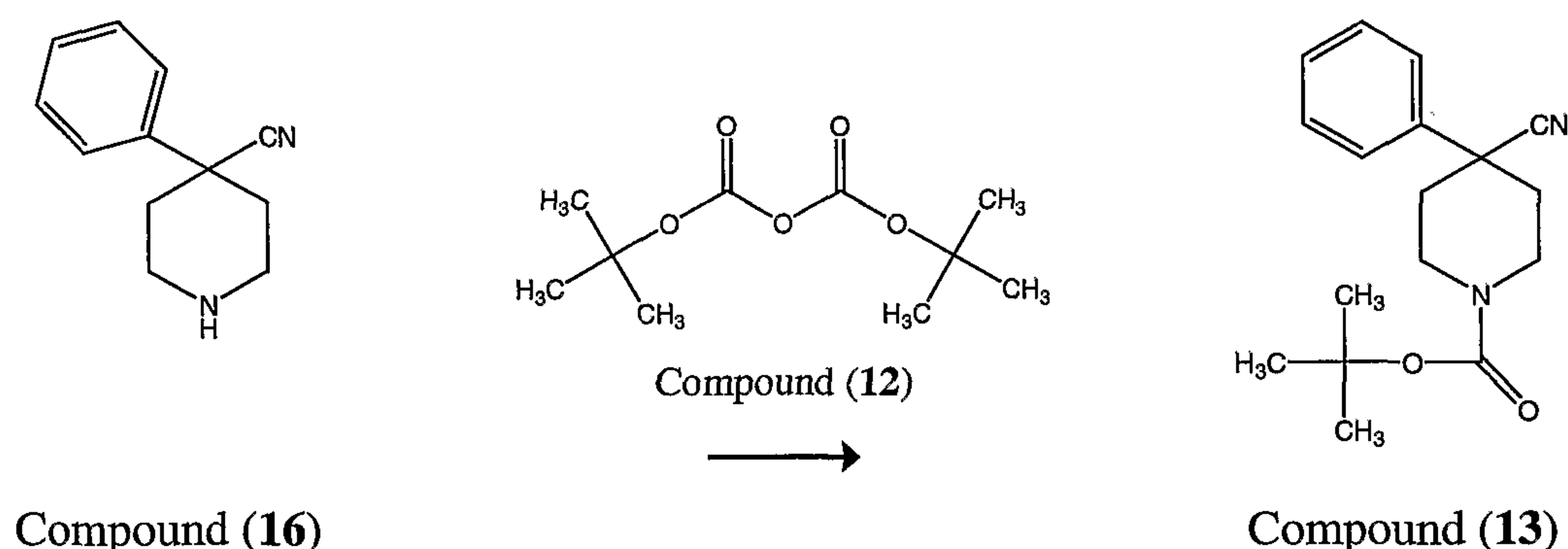
Scheme 12
