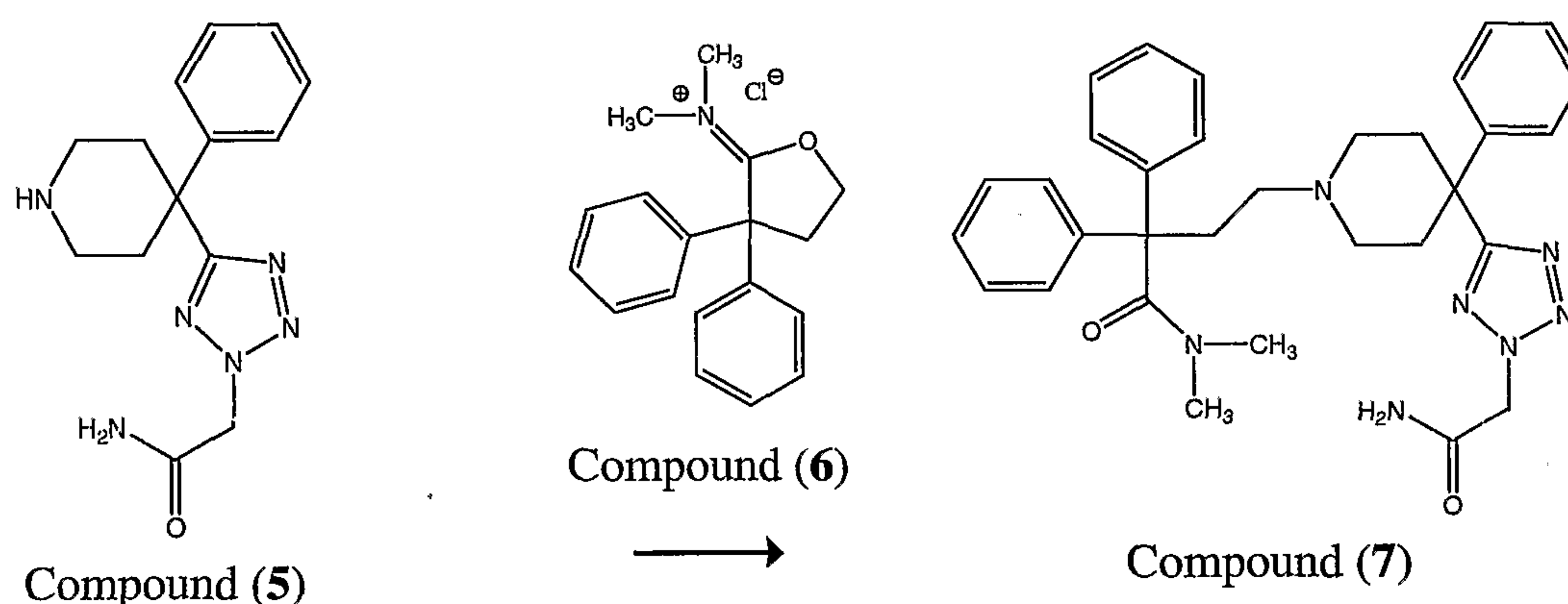
Scheme 30
