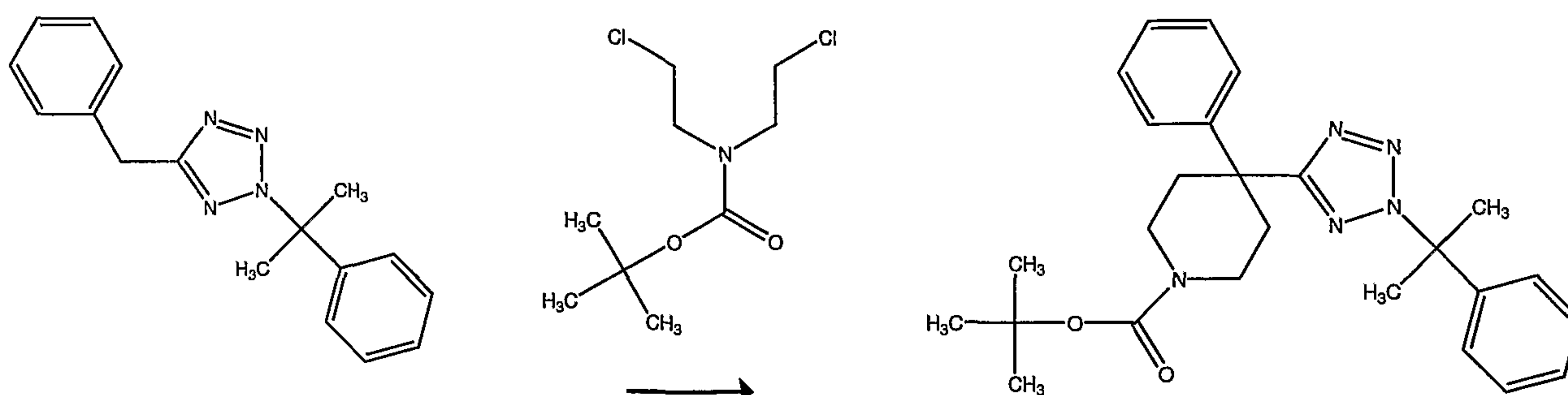
Scheme 20
