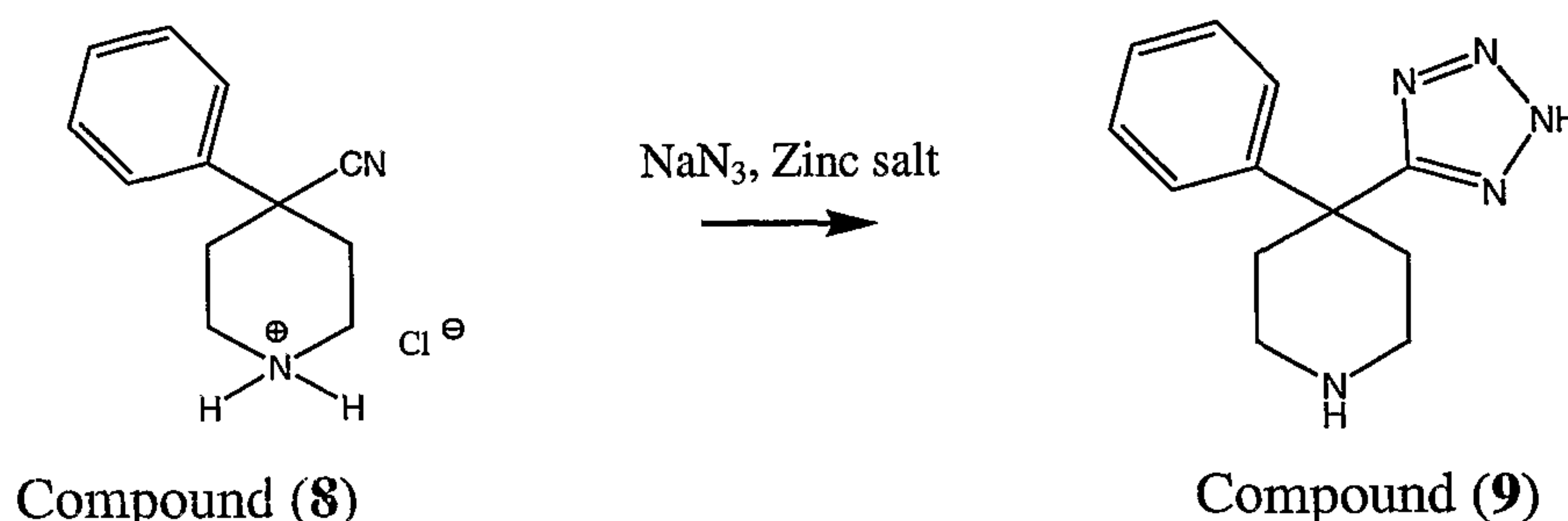
Scheme 7
