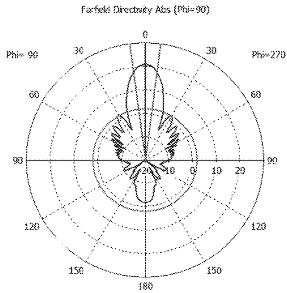
Antenna Gain Pattern
