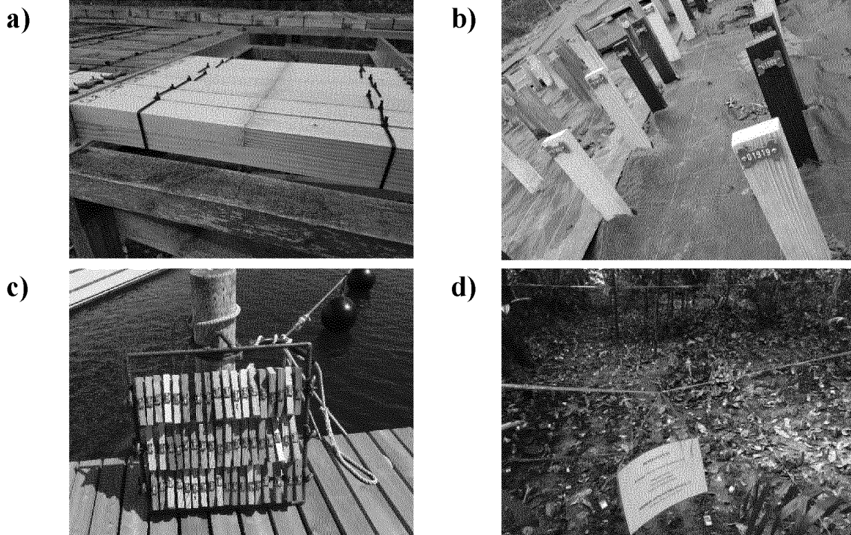
Fig. 1: Durability field testing according to use classes (UC) 3, 4, and 5 of EN 335, 2013 – a) above ground in Germany (bundle), b) in-ground (stakes, EN 252) in Germany, c) in marine environment in Denmark and d) in-ground (stakes) against wood vermin in Indonesia.
