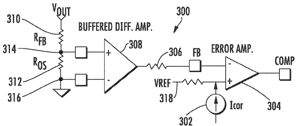
FIG. 3 (PRIOR ART)
