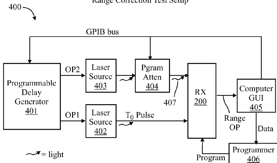
Range Correction Test Setup
