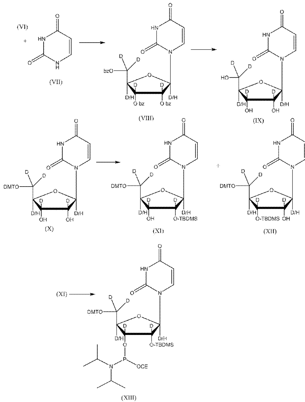
Figure 3: Scheme 2
