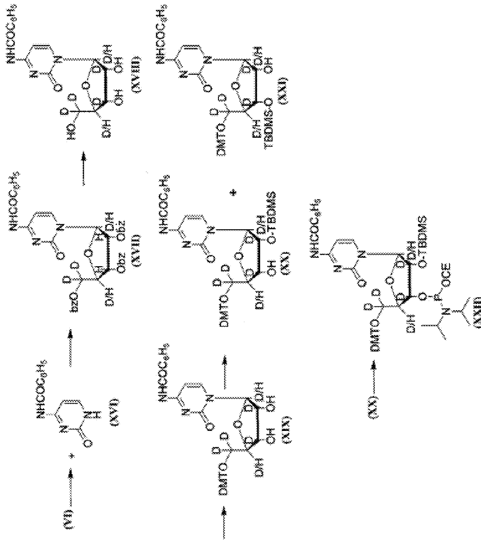
Figure 5: Scheme 4
