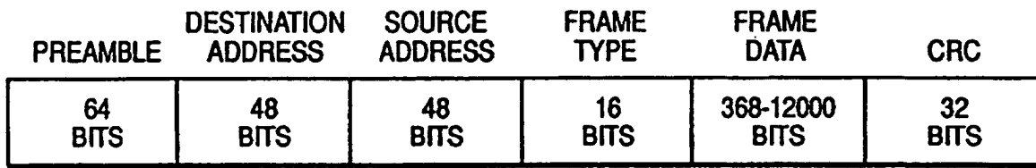
ETHERNET FRAME FORMAT
