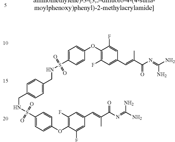
Compound 42: N,N'-(1,4-phenylenebis(methylene))bis[(E)-N-(diaminomethylene)-3-(3,5-difluoro-4-(4-sulfamoylphenoxy)phenyl)-2-methylacrylamide]
