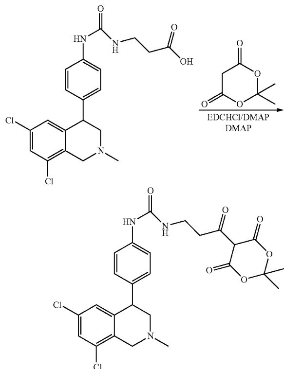
Intermediate 40.3: 1-(4-(6,8-dichloro-2-methyl-1,2,3,4-tetrahydroisoquinolin-4-yl)phenyl)-3-(3-(2,2-dimethyl-4,6-dioxo-1,3-dioxan-5-yl)-3-oxopropyl)urea
