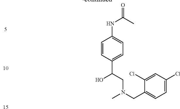
Intermediate 30.5: N-(4-(2-((2,4-dichlorobenzyl)(methyl)amino)-1-hydroxyethyl)phenyl)acetamide
