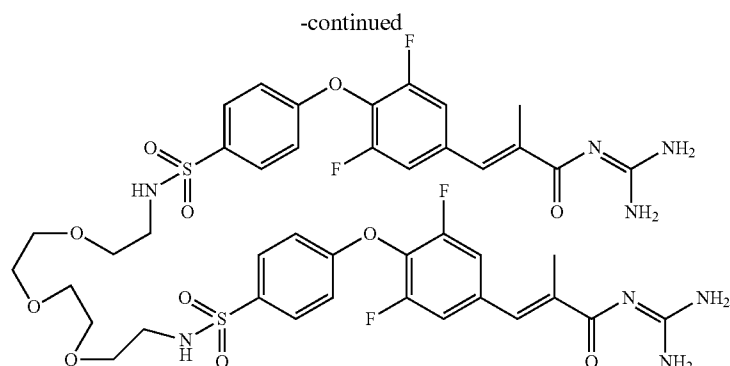
Compound 44 N,N'-(2,2'-(2,2'-oxybis(ethane-2,1-diyl))bis(oxy))bis(ethane-2,1-diyl)bis[(E)-N-(diaminomethylene)-3-(3,5-difluoro-4-(4-sulfamoylphenoxy)phenyl)-2-methylacrylamide]
