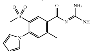
Eniporide
