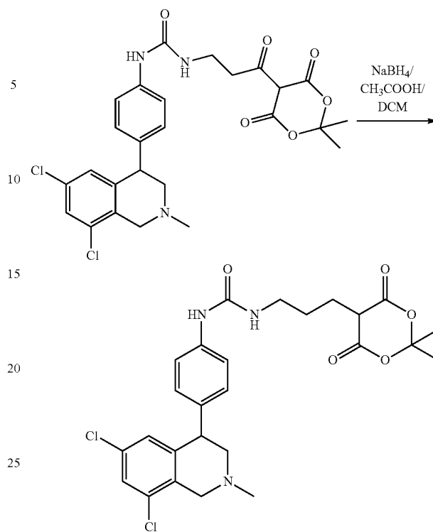
Intermediate 40.4: 1-(4-(6,8-dichloro-2-methyl-1,2,3,4-tetrahydroisoquinolin-4-yl)phenyl)-3-(3-(2,2-dimethyl-4,6-dioxo-1,3-dioxan-5-yl)propyl)urea
