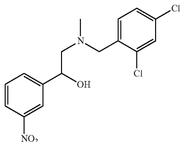
Intermediate 31.3: 2-((2,4-dichlorobenzyl)(methyl)amino)-1-(3-nitrophenyl)ethanol
