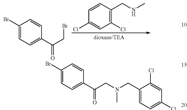
Intermediate 10.2: 1-(4-bromophenyl)-2-((2,4-dichlorobenzyl)(methyl)amino)ethanone
