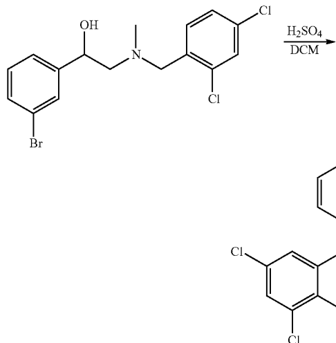
Intermediate 1.4: 4-(3-bromophenyl)-6,8-dichloro-2-methyl-1,2,3,4-tetrahydroisoquinoline
