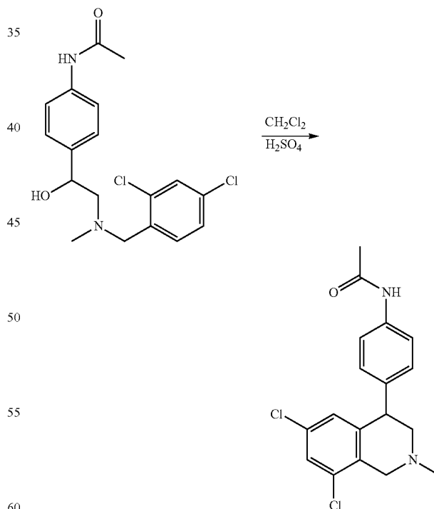
Intermediate 30.6: N-(4-(6,8-dichloro-2-methyl-1,2,3,4-tetrahydroisoquinolin-4-yl)phenyl)acetamide
