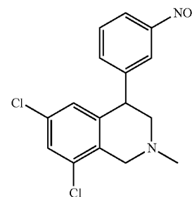
Intermediate 31.4: 6,8-dichloro-2-methyl-4-(3-nitrophenyl)-1,2,3,4-tetrahydroisoquinoline
