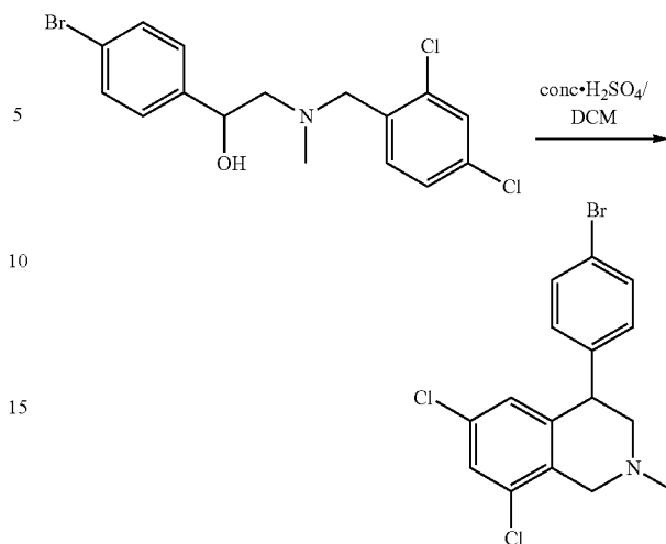
Intermediate 10.4: 4-(4-bromophenyl)-6,8-dichloro-2-methyl-1,2,3,4-tetrahydroisoquinoline
