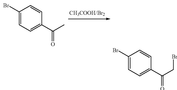
Intermediate 10.1: 2-bromo-1-(4-bromophenyl)ethanone
