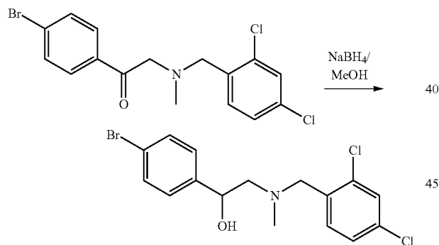
Intermediate 10.3: 2-((2,4-dichlorobenzyl)(methyl)amino)-1-(4-bromophenyl)ethanol
