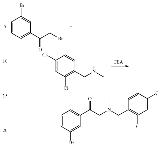
Intermediate 1.2: 1-(3-bromophenyl)-2-((2,4-dichlorobenzyl)(methyl)amino)ethanone
