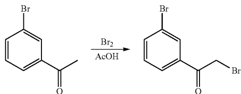
Intermediate 1.1: 2-bromo-1-(3-bromophenyl)ethanone
