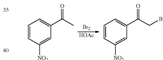
Intermediate 31.1: 2-bromo-1-(3-nitrophenyl)ethanone
