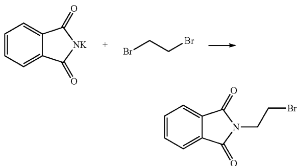
Intermediate 1.7: 2-(2-bromoethyl)isoindoline-1,3-dione
