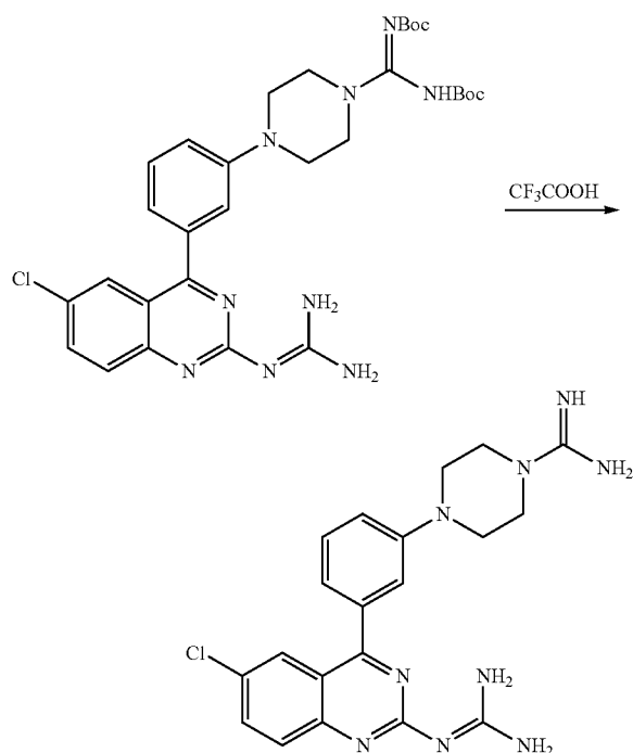
Compound 60: 4-(3-(6-chloro-2-(diaminomethyleneamino)quinazolin-4-yl)phenyl)piperazine-1-carboximidamide
