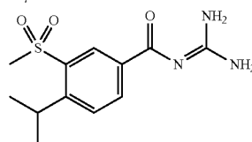
Cariporide
