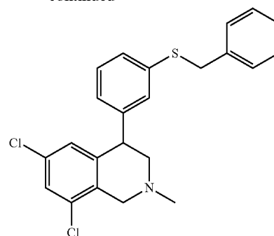
Intermediate 1.5: 4-(3-(benzylthio)phenyl)-6,8-dichloro-2-methyl-1,2,3,4-tetrahydroisoquinoline
