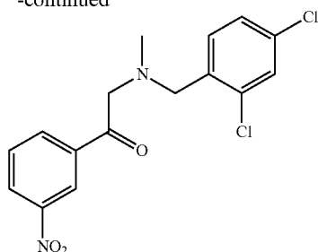
Intermediate 31.2: 2-((2,4-dichlorobenzyl)(methyl)amino)-1-(3-nitrophenyl)ethanone
