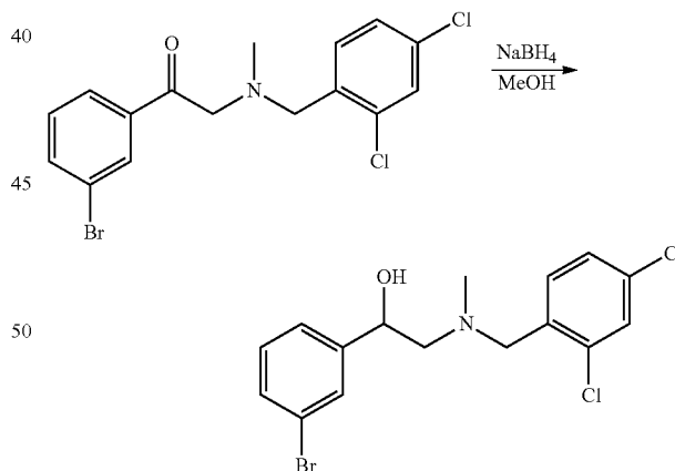
Intermediate 1.3: 1-(3-bromophenyl)-2-((2,4-dichlorobenzyl)(methyl)amino)ethanol
