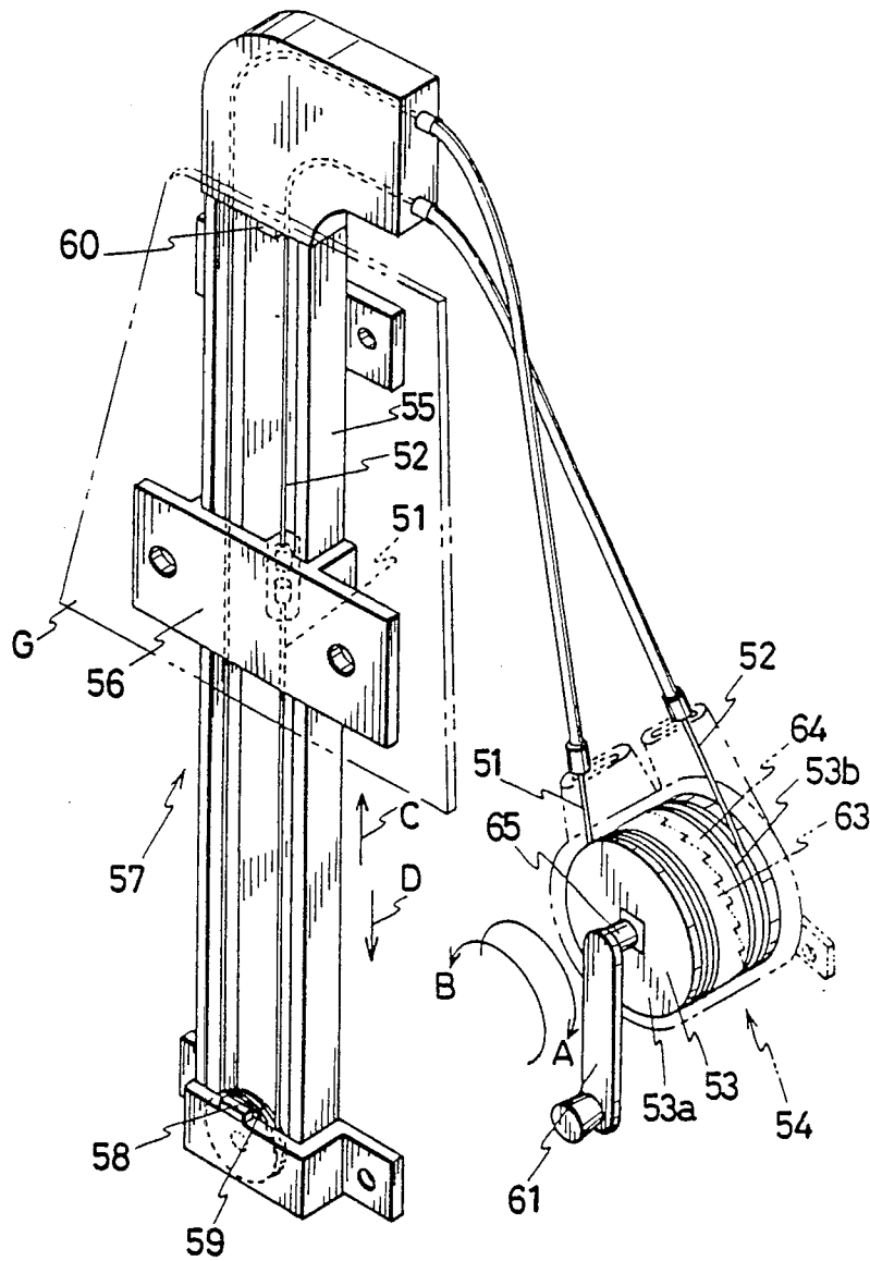
Fig. 14 (PRIOR ART)
