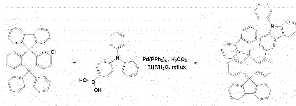
[Compound A]
