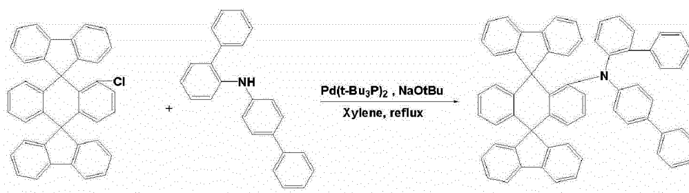
[Compound A]
