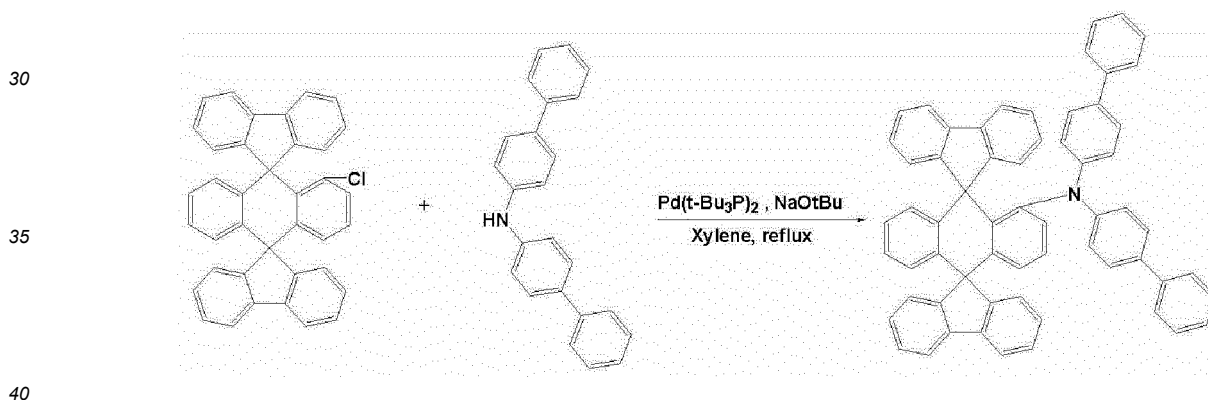
[Compound A]
