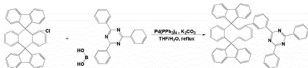
[Compound A]
