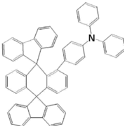
[Compound 2]
