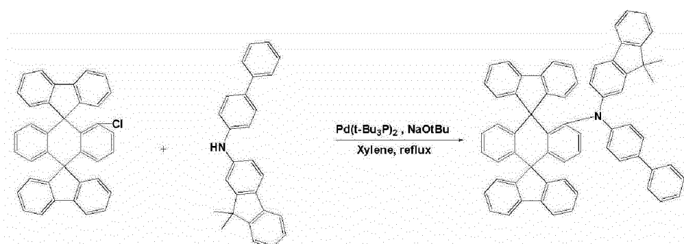
[Compound A]
