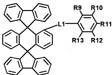
[Chemical Formula 1-3]
