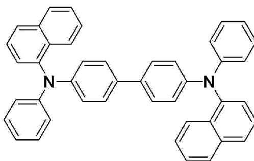
[NPB]
