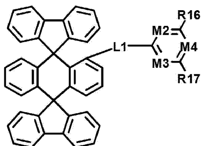
[Chemical Formula 1-5]
