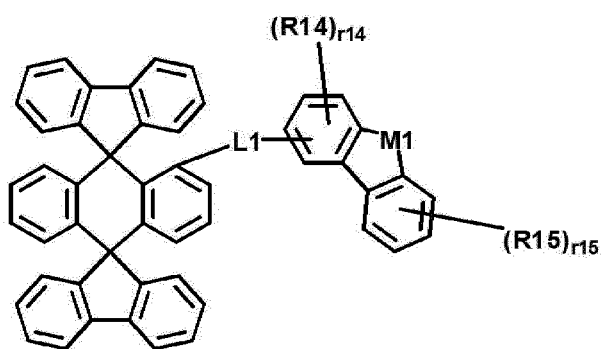
[Chemical Formula 1-5]
