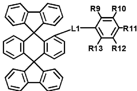
[Chemical Formula 1-4]
