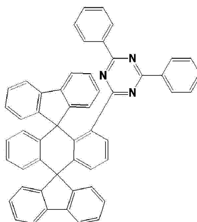
[Compound 4]
