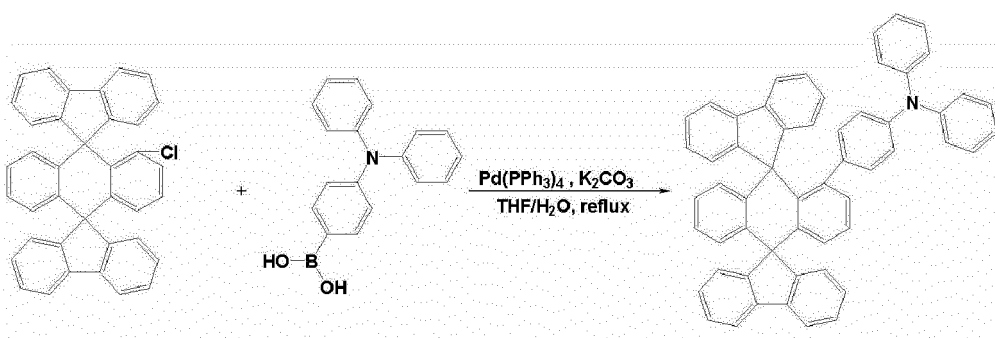
[Compound A]
