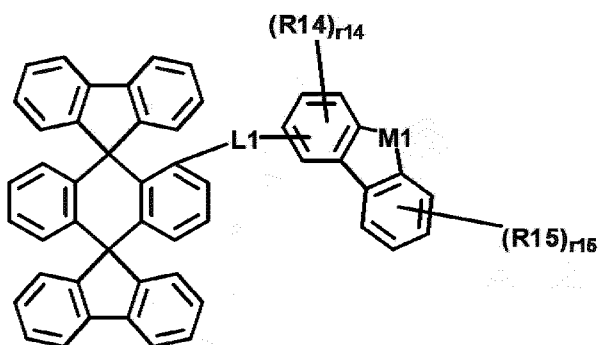
[Chemical Formula 1-4]
