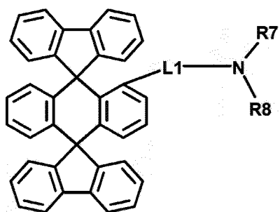
[Chemical Formula 1-2]
