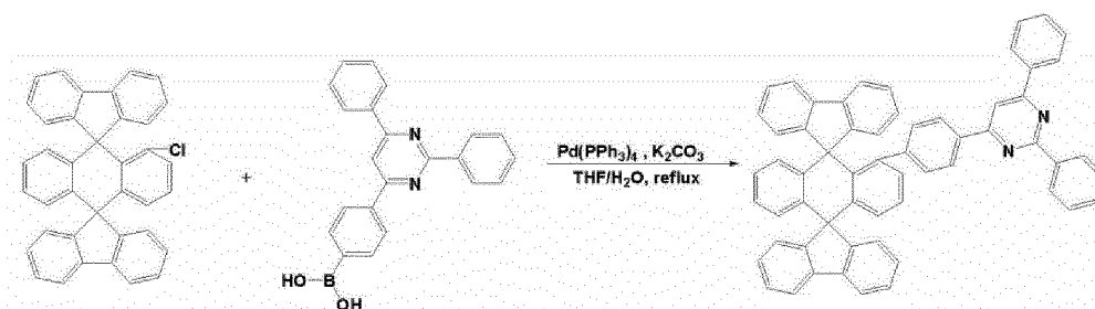
[Compound A]
