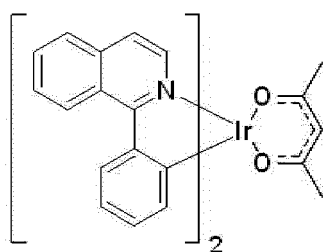
[(piq) 2 Ir(acac)]
