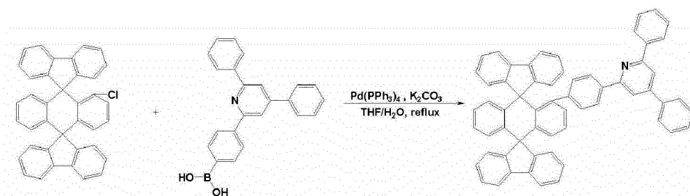
[Compound A]
