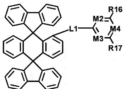
[Chemical Formula 1-5]
