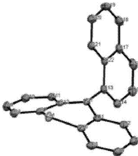
1-naphthalene-10-phenothiazine
