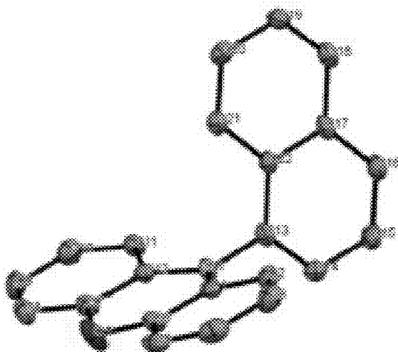
1-naphthalene-10-phenoxazine
