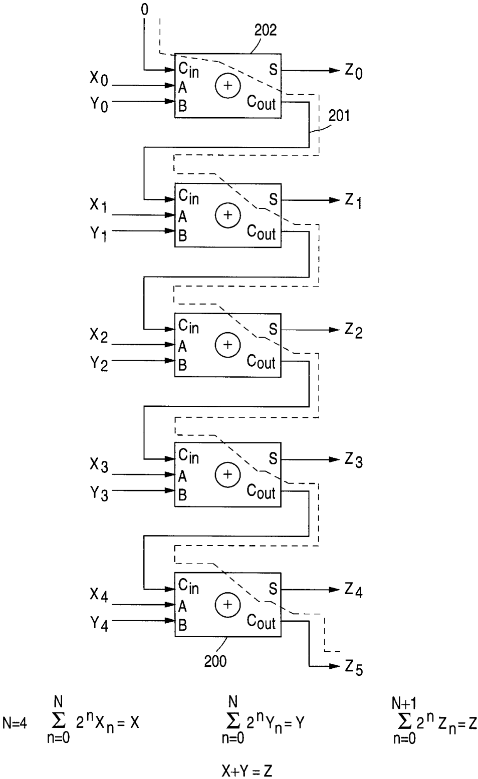
FIGURE 2 (PRIOR ART)
