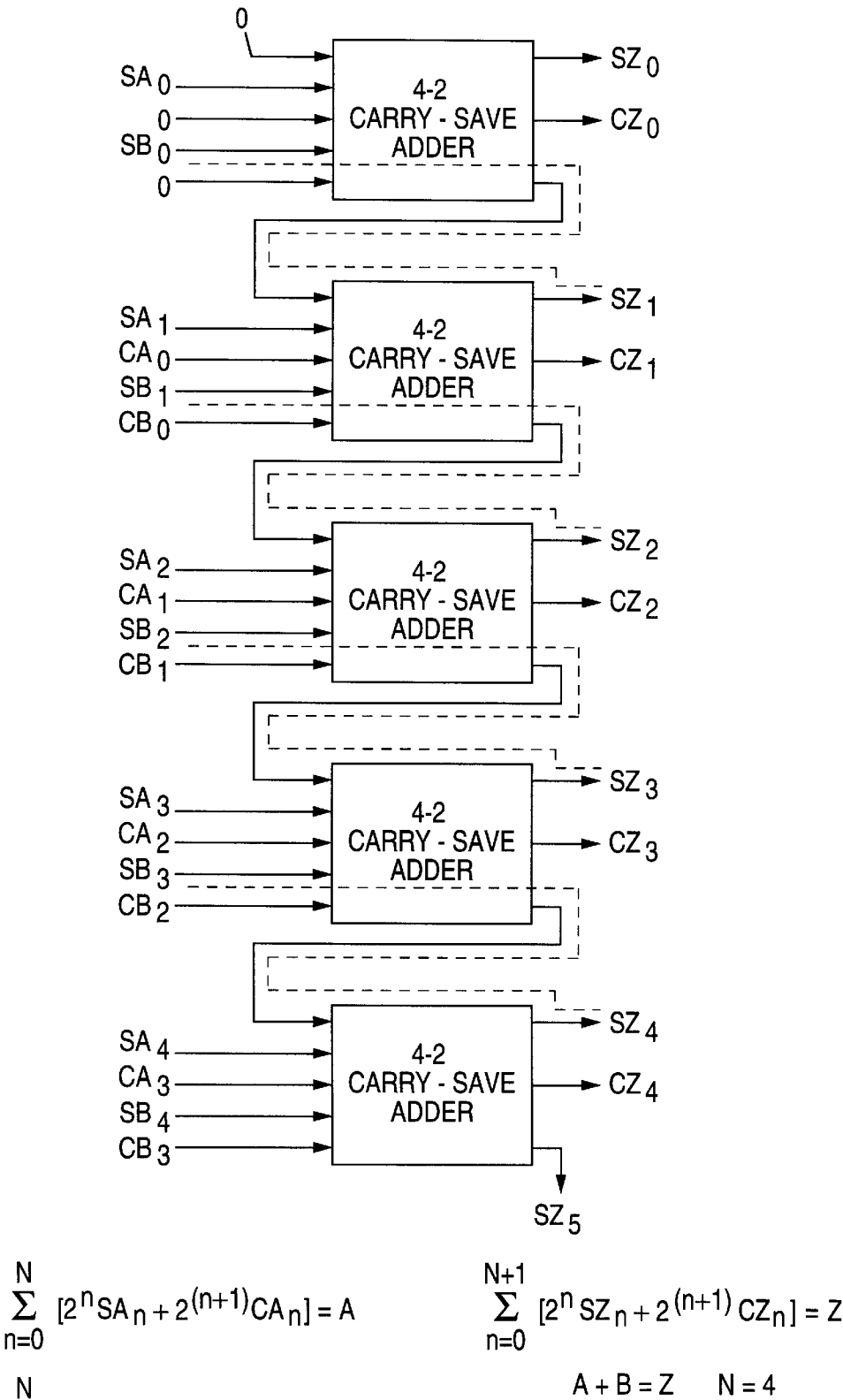
FIGURE 4 (PRIOR ART)
