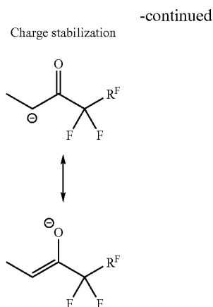
Scheme 1. Effect of Carbonyl Substitution/Insertion.
