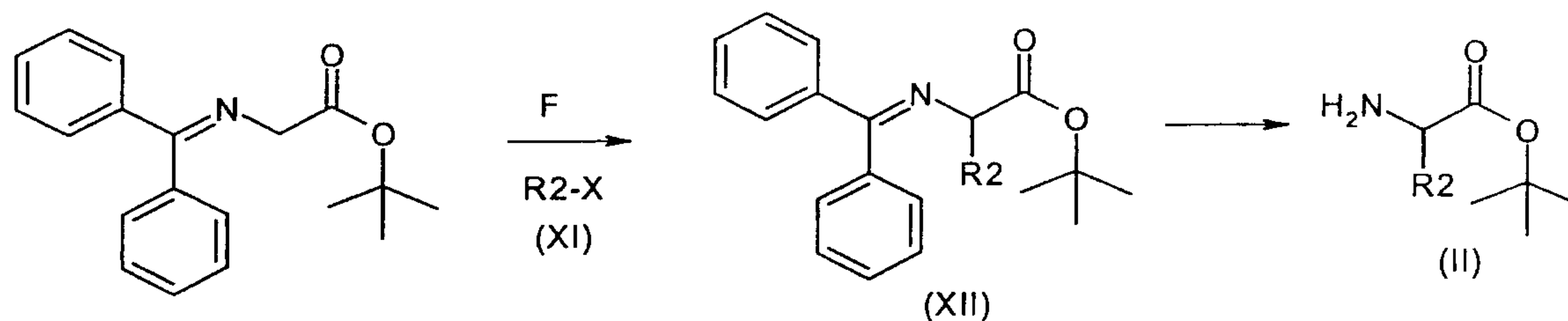
Scheme 4
