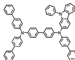
HT36
