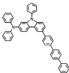
HT25
