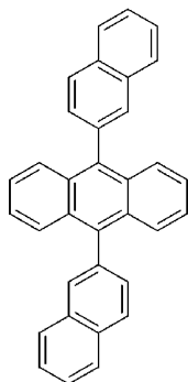
ADN
