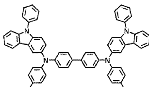
HT29
