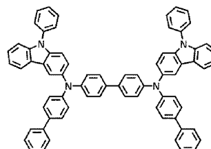
HT33
