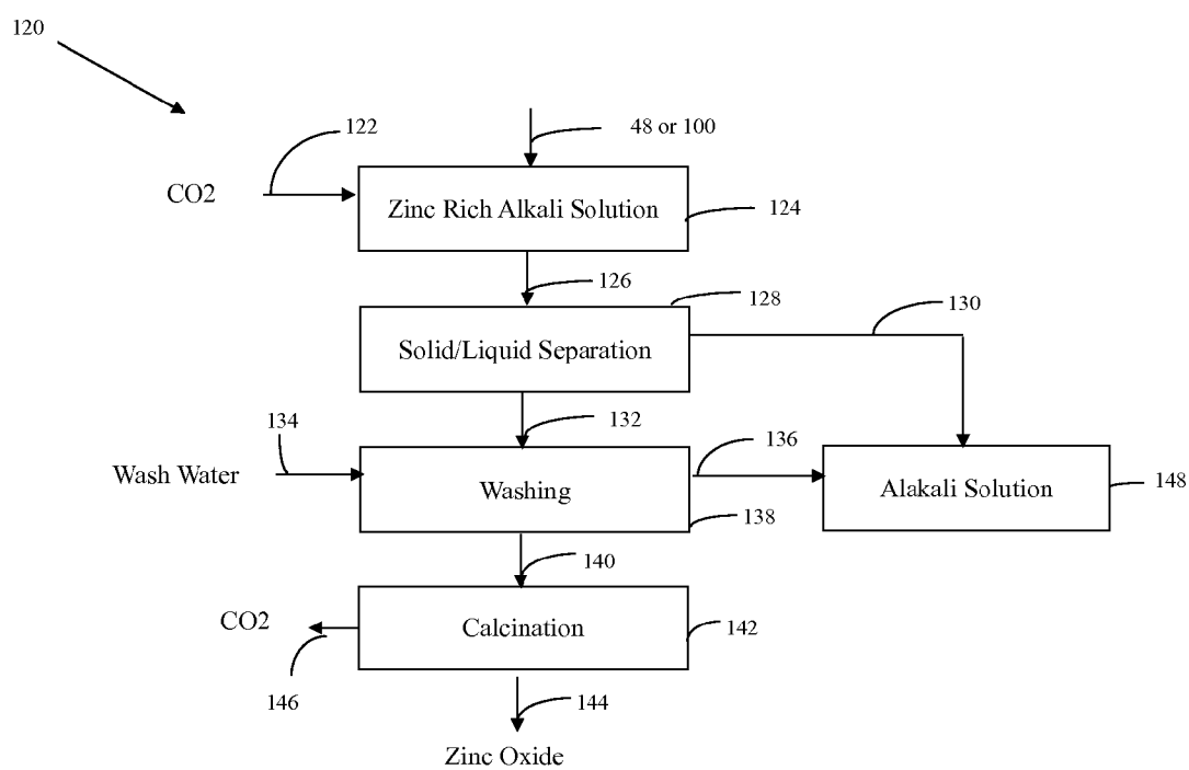
Figure 3: Zinc recovery from alkaline leach solutions
