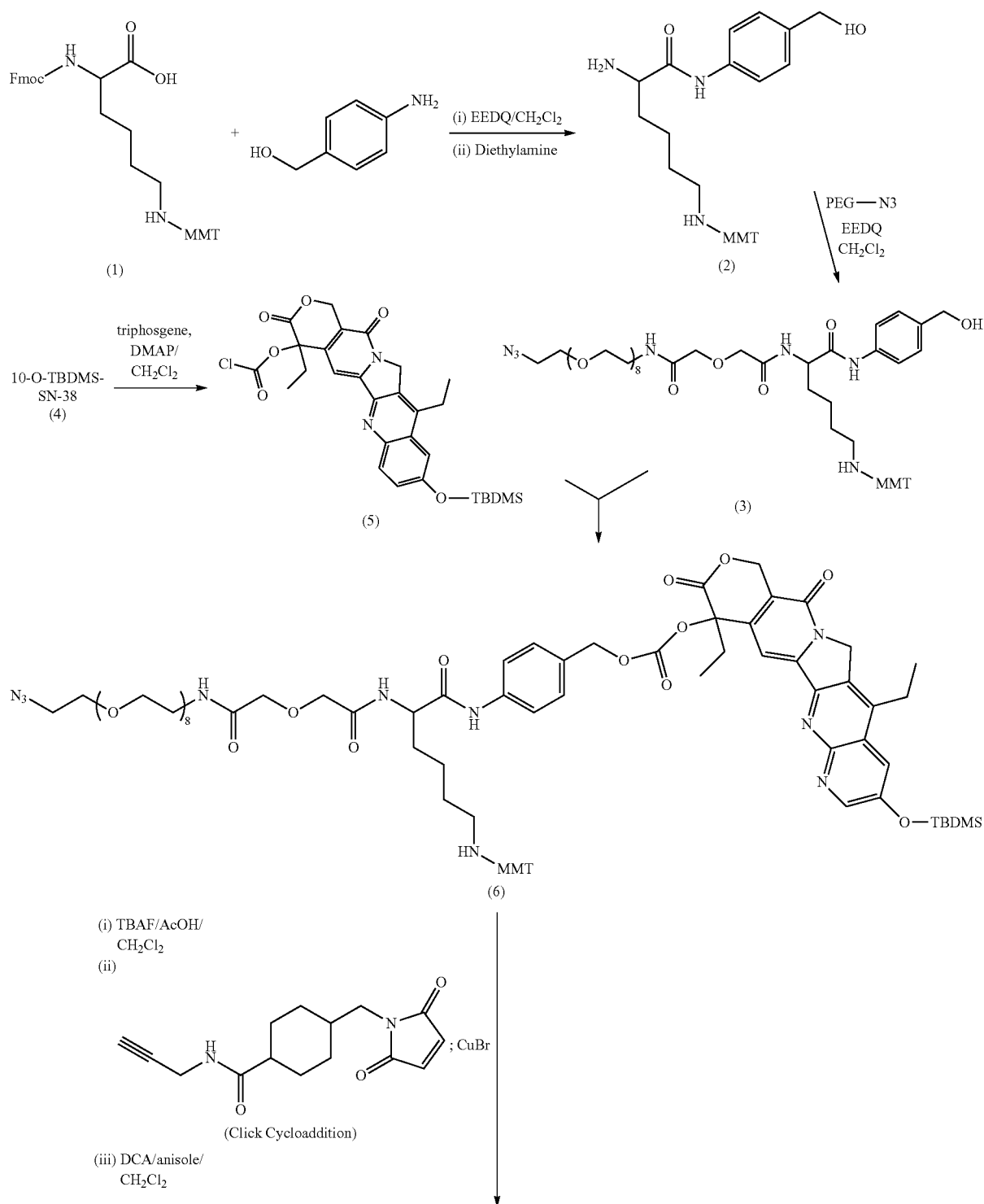
Scheme-3: Preparation of CL2A-SN-38
