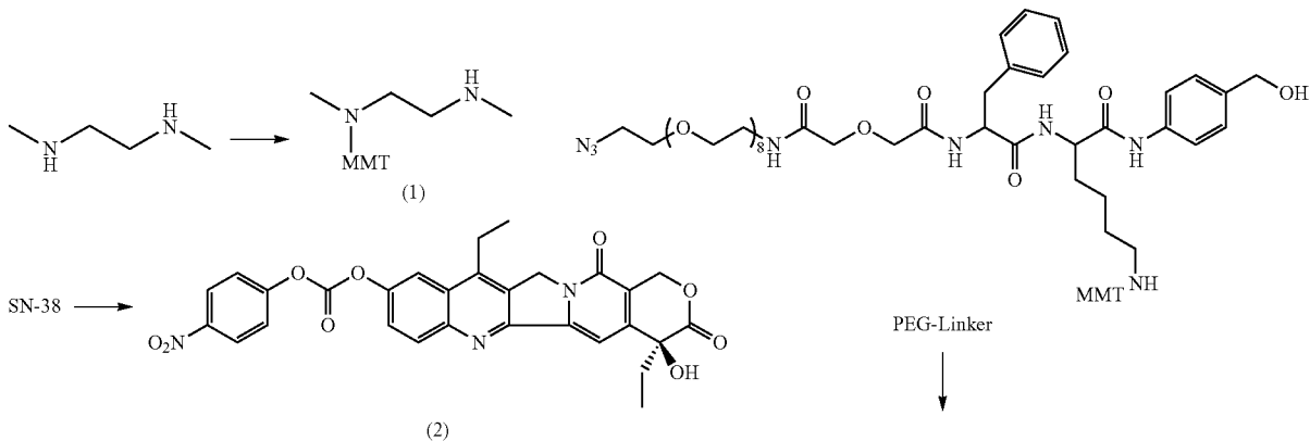
Scheme-4: Preparation of CL2E-SN-38
