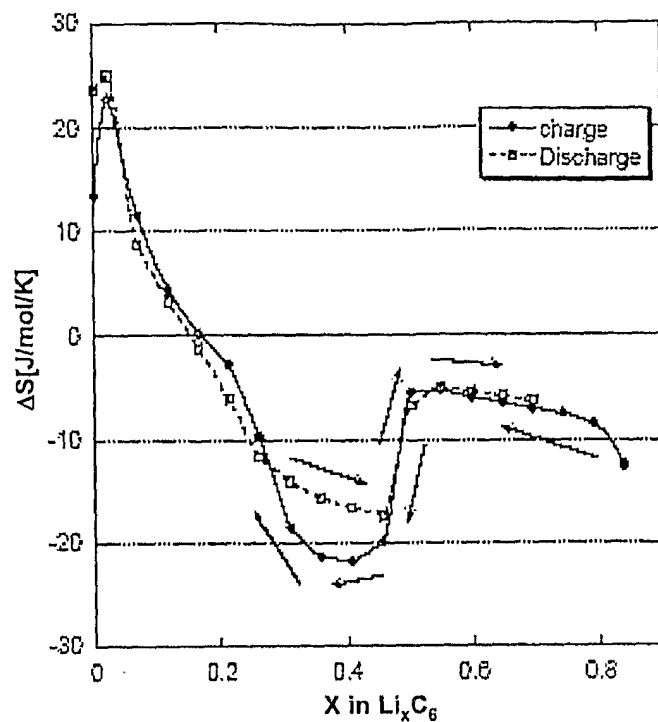
Entropy of Li intercalation during charge and discharge of coke HTT at 2600°C
