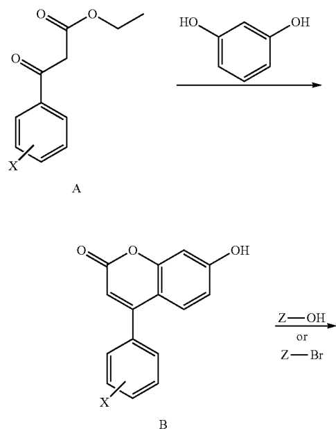
Scheme 1: Exemplary preparation of a compound of formula (C)
