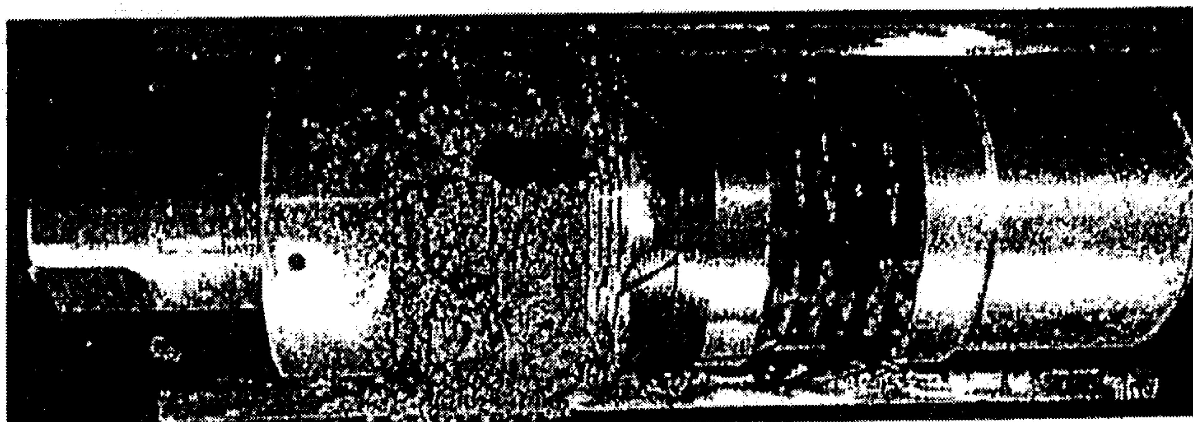
FIGURE 3G: assembly as tested, post-test with sand
