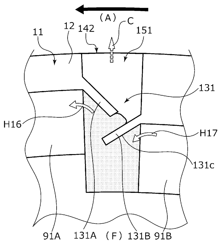
Fig. 10 ROTATIONAL DIRECTION OF ROTATING SEAL RING
