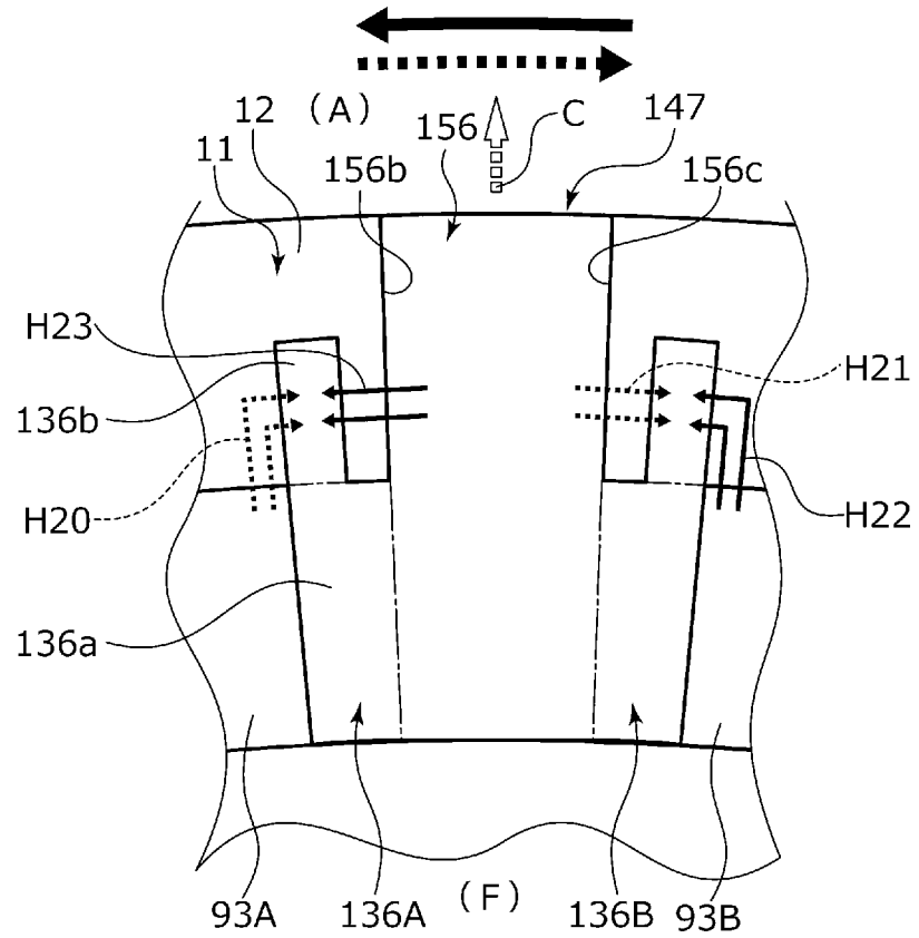
Fig. 15 ROTATIONAL DIRECTION OF ROTATING SEAL RING
