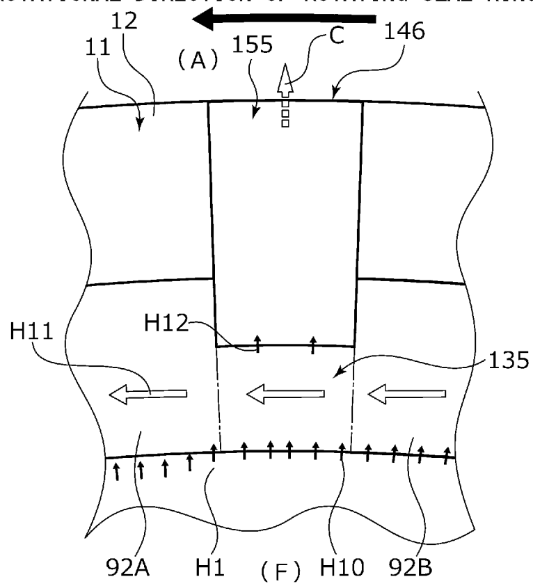
Fig. 14 ROTATIONAL DIRECTION OF ROTATING SEAL RING
