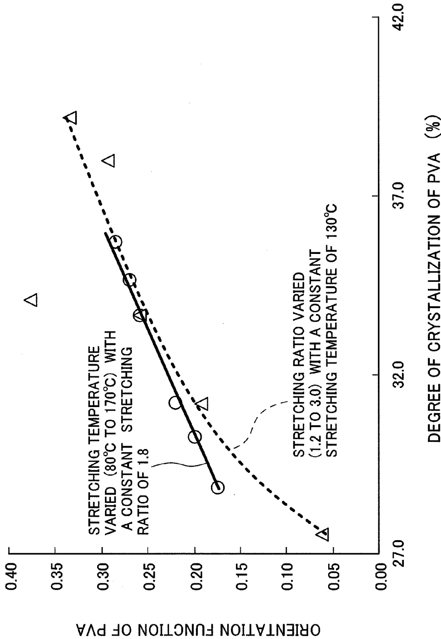
FIG. 24 DEGREE OF CRYSTALLIZATION AND ORIENTATION OF PVA
