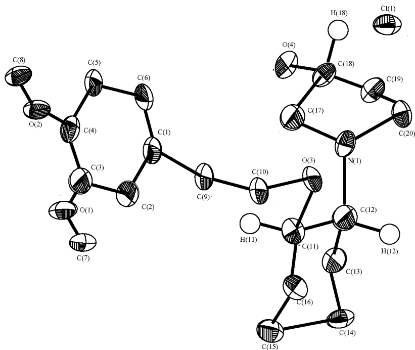
X-Ray Structure of Compound 1
