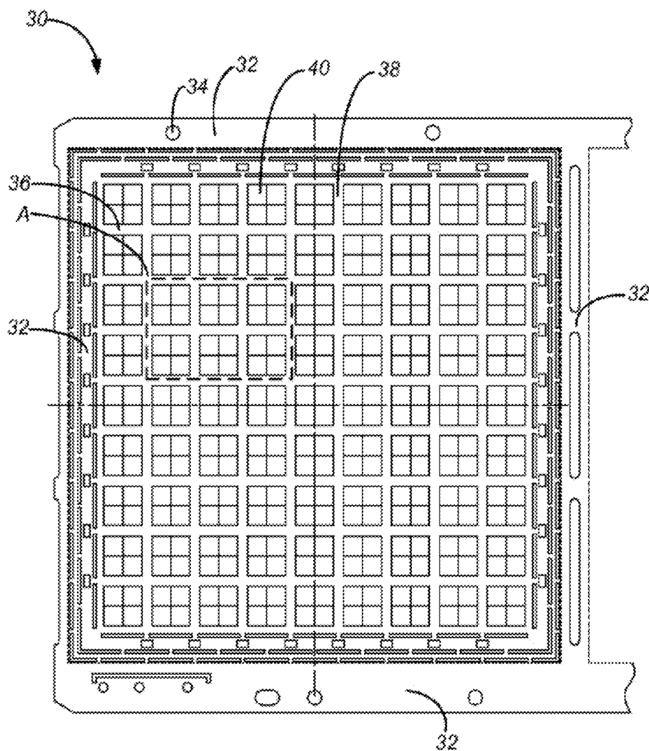
FIG. 2 (PRIOR ART)
