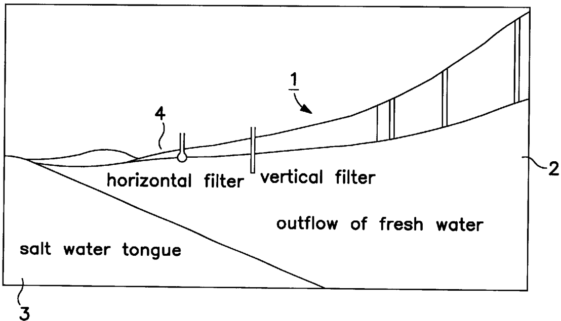
Schematic placing in coastal profile
