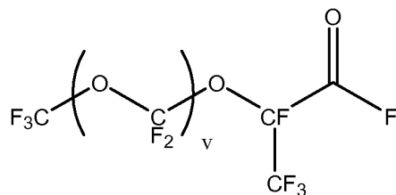
Compound D3
