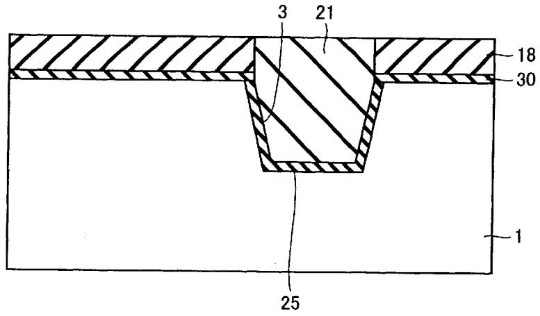
FIG.34 PRIOR ART
