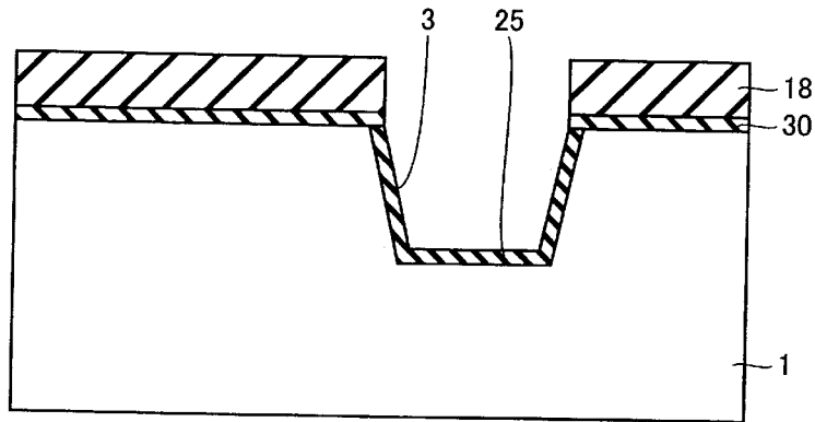
FIG.32 PRIOR ART
