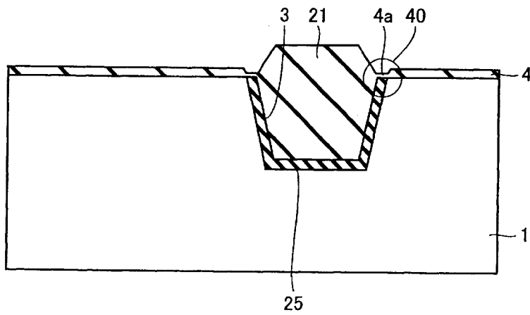
FIG.36 PRIOR ART
