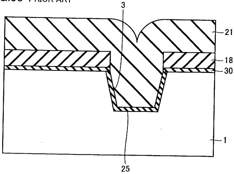
FIG.33 PRIOR ART
