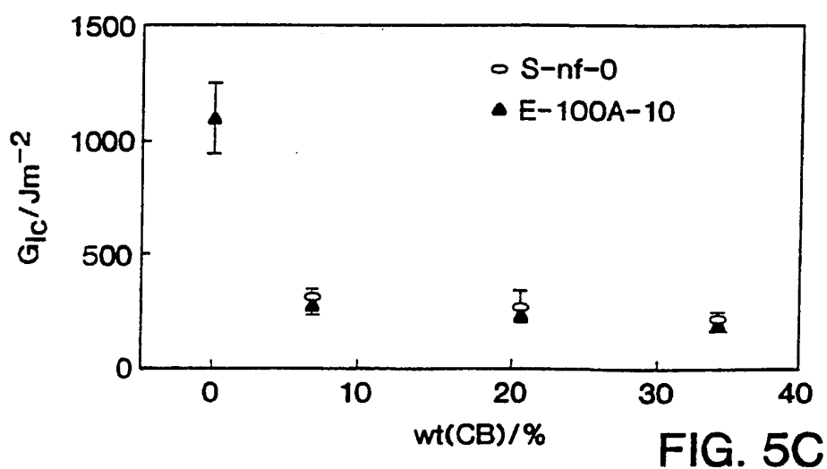
Variation of fraction energy, G_{IC} , with weight percentage, wt(CB) , of carbon black (a) R-nf-0 and R-NH 2 -20(BA), (b) S-nf-0 and S-NH 2 -20(BA) and (c) S-nf-0 and E-100A-10
