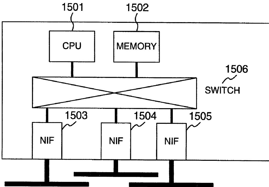
CONFIGURATION EXAMPLE OF HA DEVICE AND ROUTER
