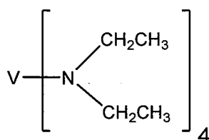
Comparative Compound 1
