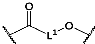
Formula L-3
