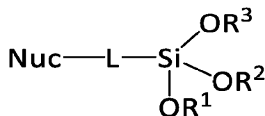
Formula C
