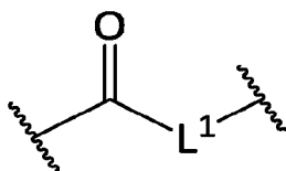
Formula L-5
