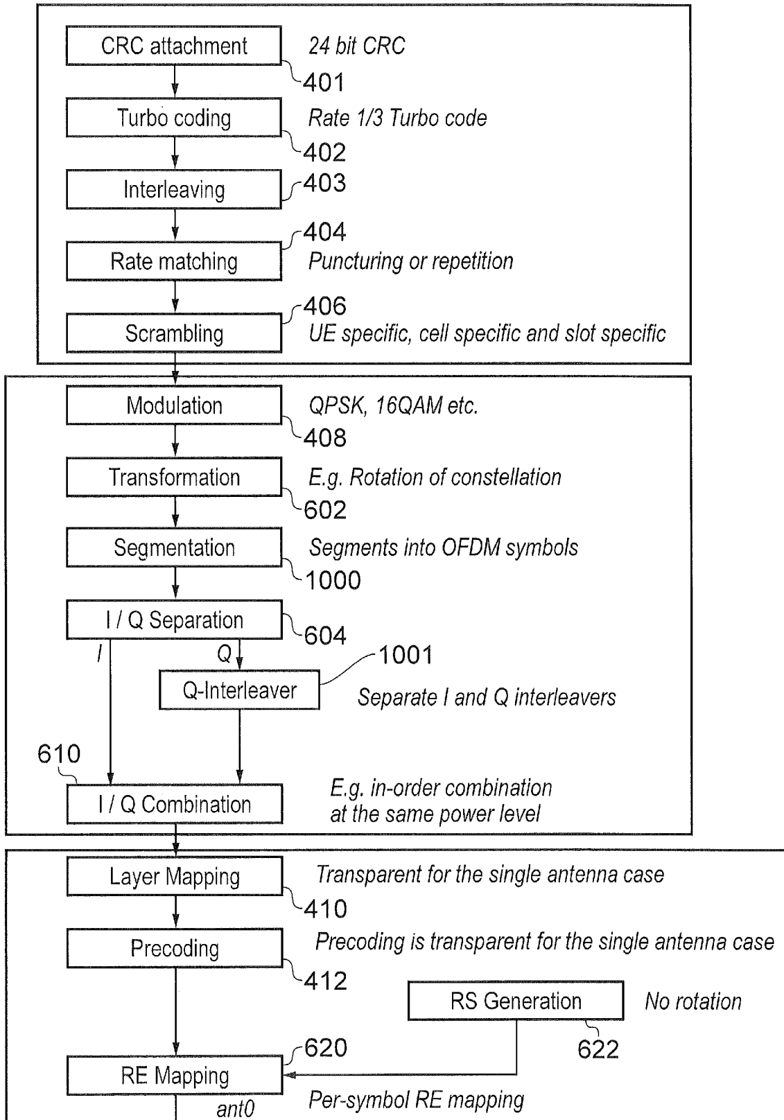
FIG. 10 Transport channel processing chain
