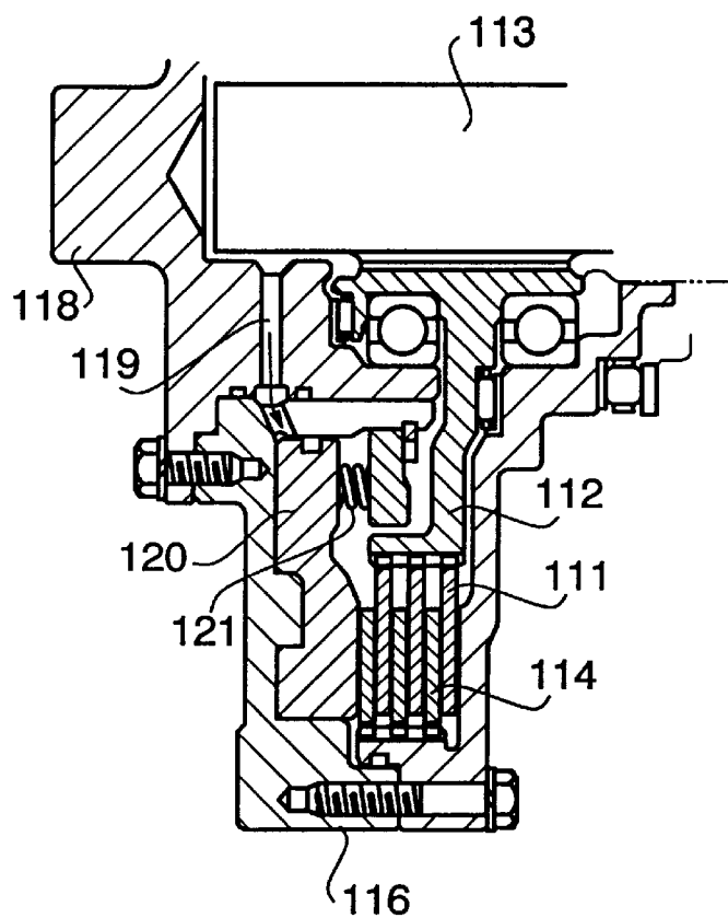
FIG. 6 PRIOR ART
