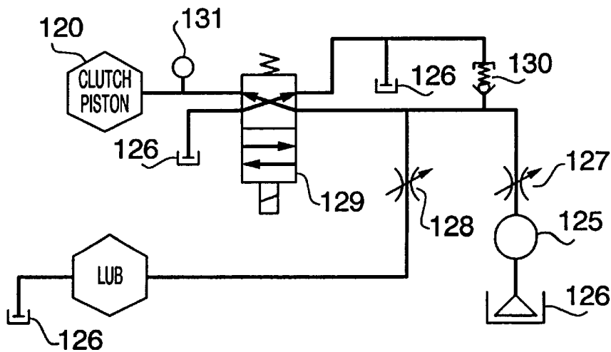
FIG. 7 PRIOR ART
