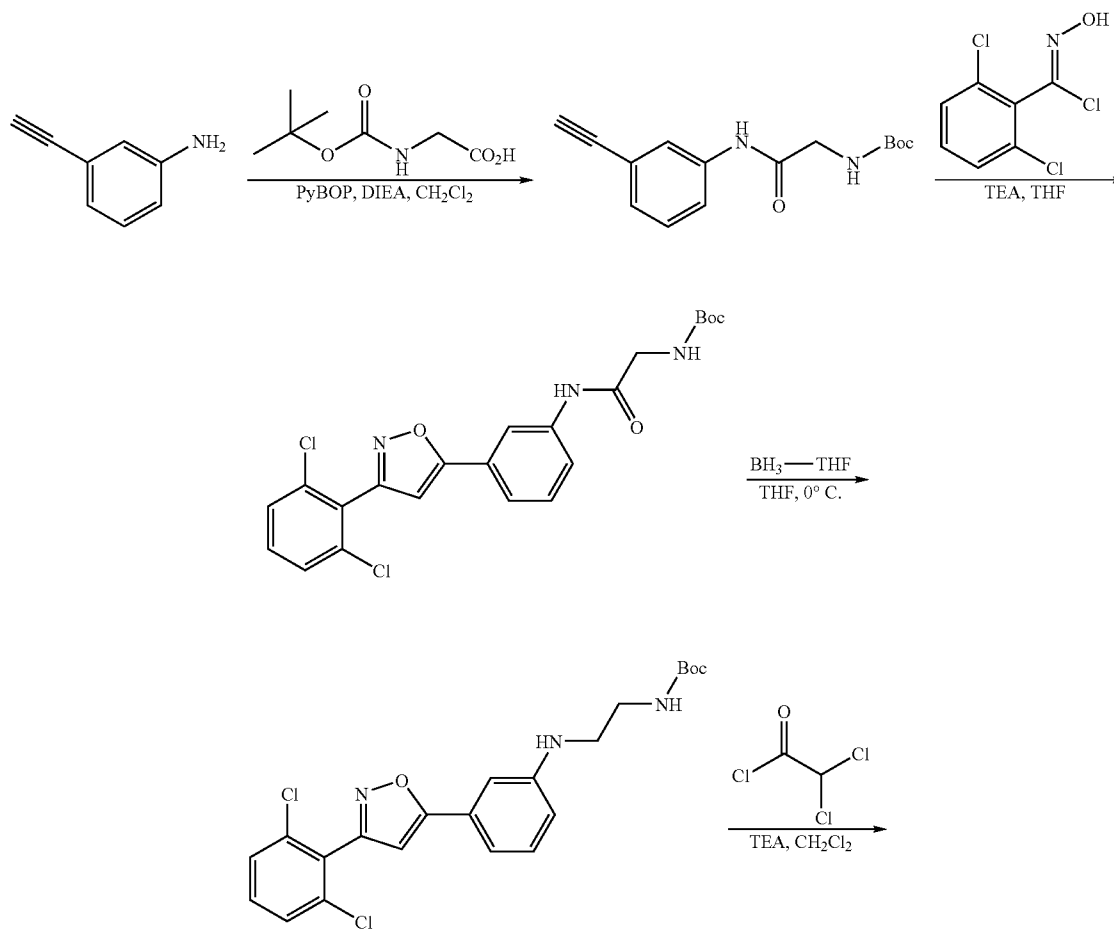
Scheme 6
