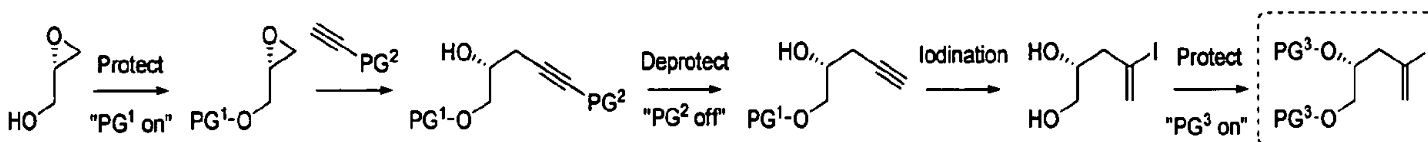
Scheme 3a: (R)-diol-protected 4-iodopent-4-ene-1,2-diol
