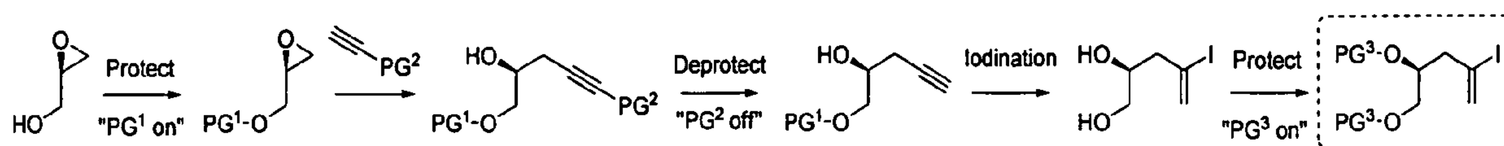
Scheme 3b: (S)-diol-protected 4-iodopent-4-ene-1,2-diol
