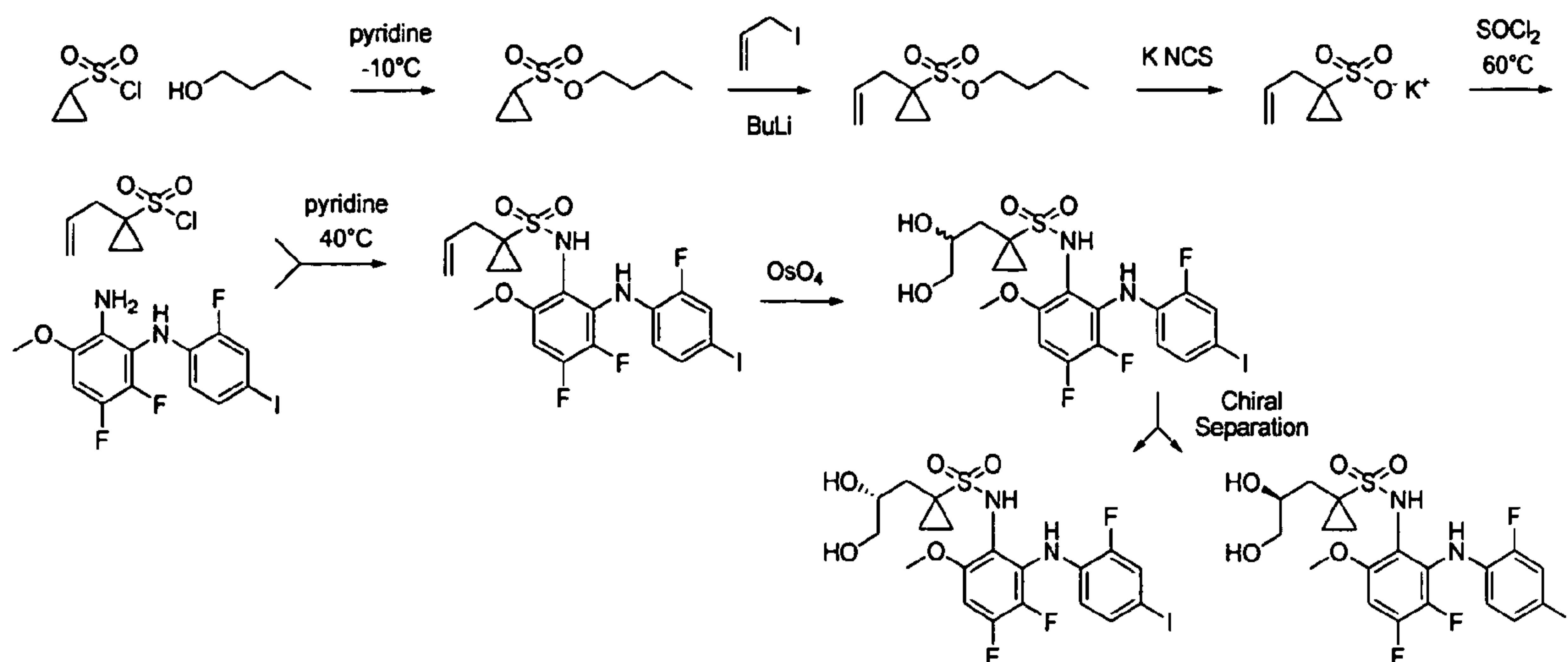
Scheme 1: Achiral synthesis of N-(3,4-difluoro-2-(2-fluoro-4-iodophenylamino)-6-methoxyphenyl)-1-(2,3-dihydroxypropyl)cyclopropane-1-sulfonamide
