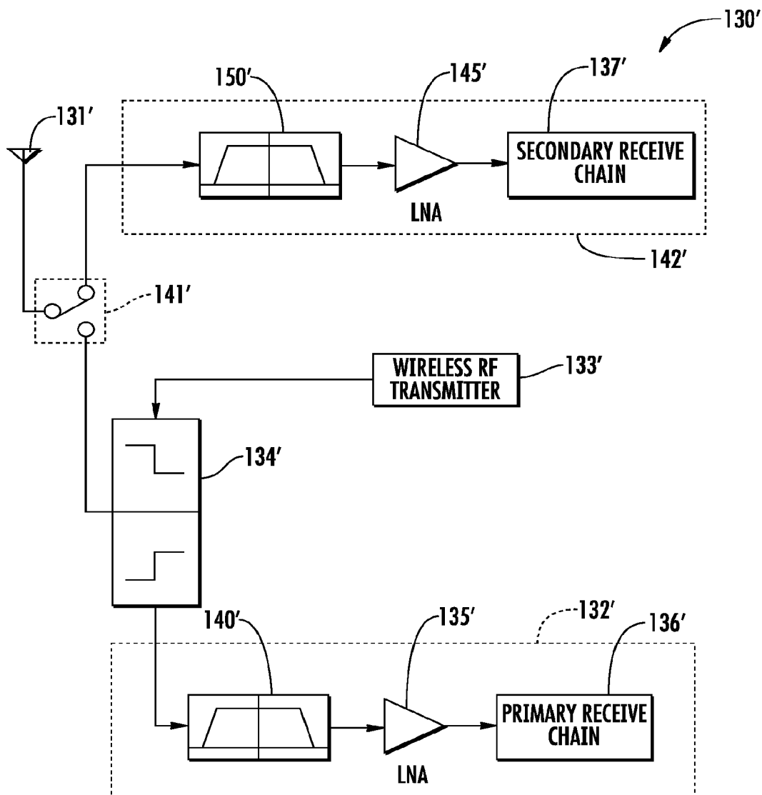
FIG. 6 (PRIOR ART)
