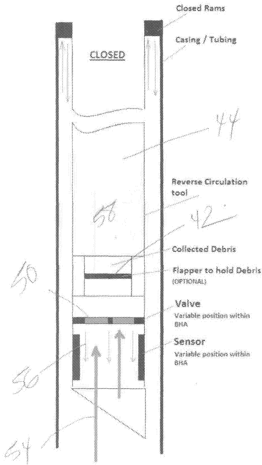
FIG. 2 - Trigger Valve - design CLOSED.PNG
